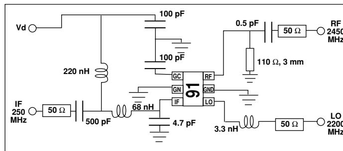
Figure 33. 800-900 MHz Cellular and ISM Band Mixer.
