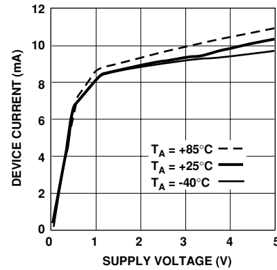
Figure 8. Device Current vs. Supply Voltage and Temperature.
