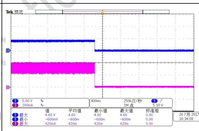
图 9, LD 至低电平 (CH1:VLD CH3:Iout)
