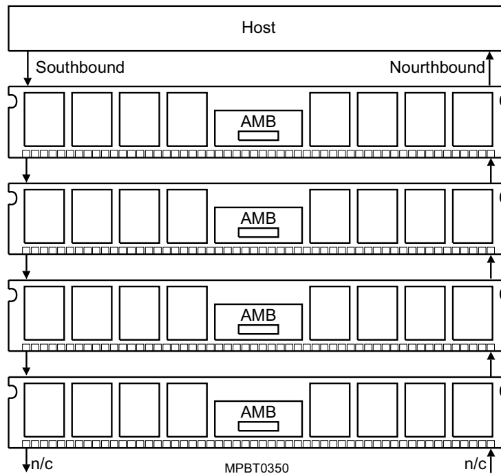
Block Diagram of Channel Southbound and Northbound Paths
