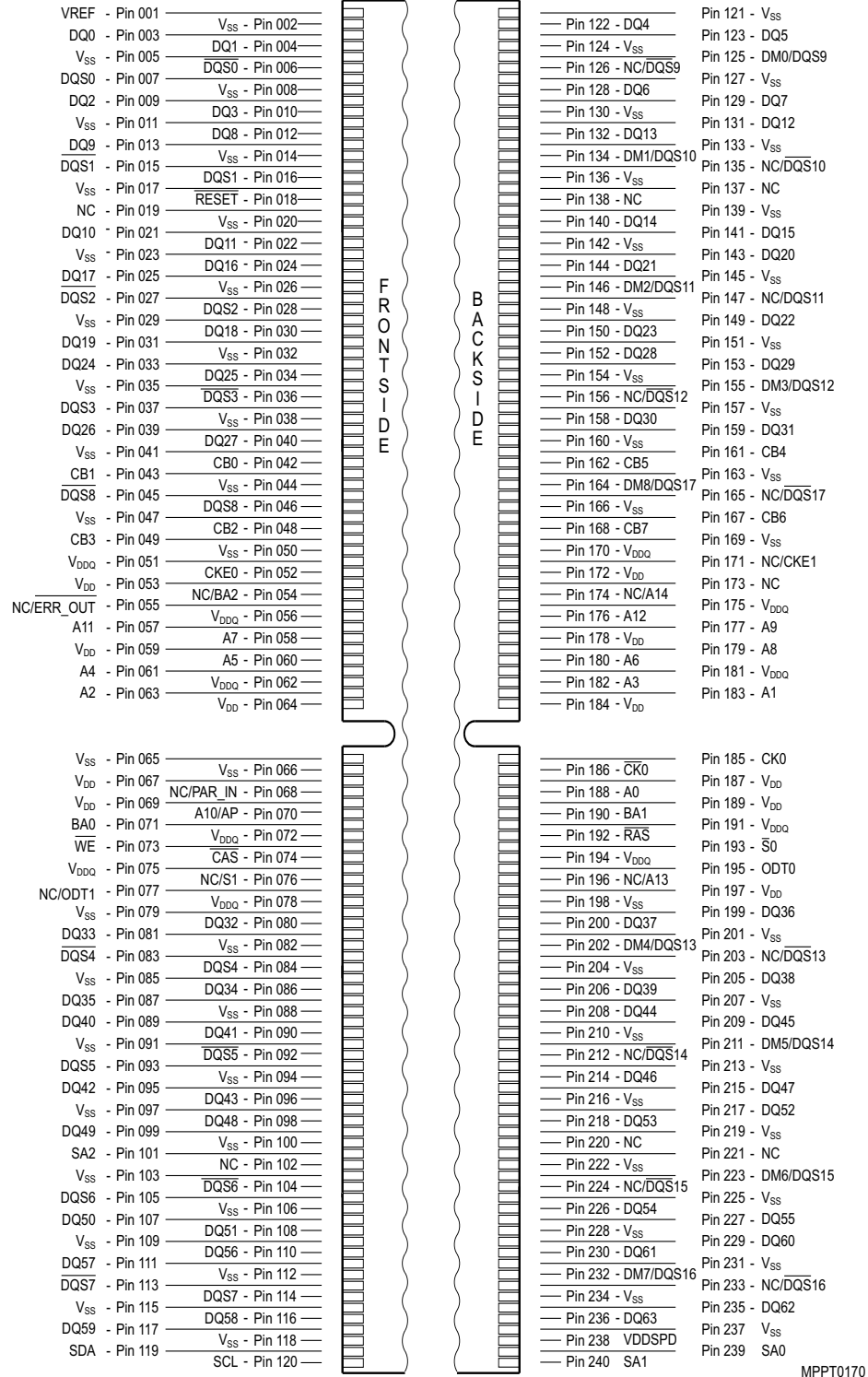
FIGURE 1 Pin Configuration for RDIMM (240 pins)
