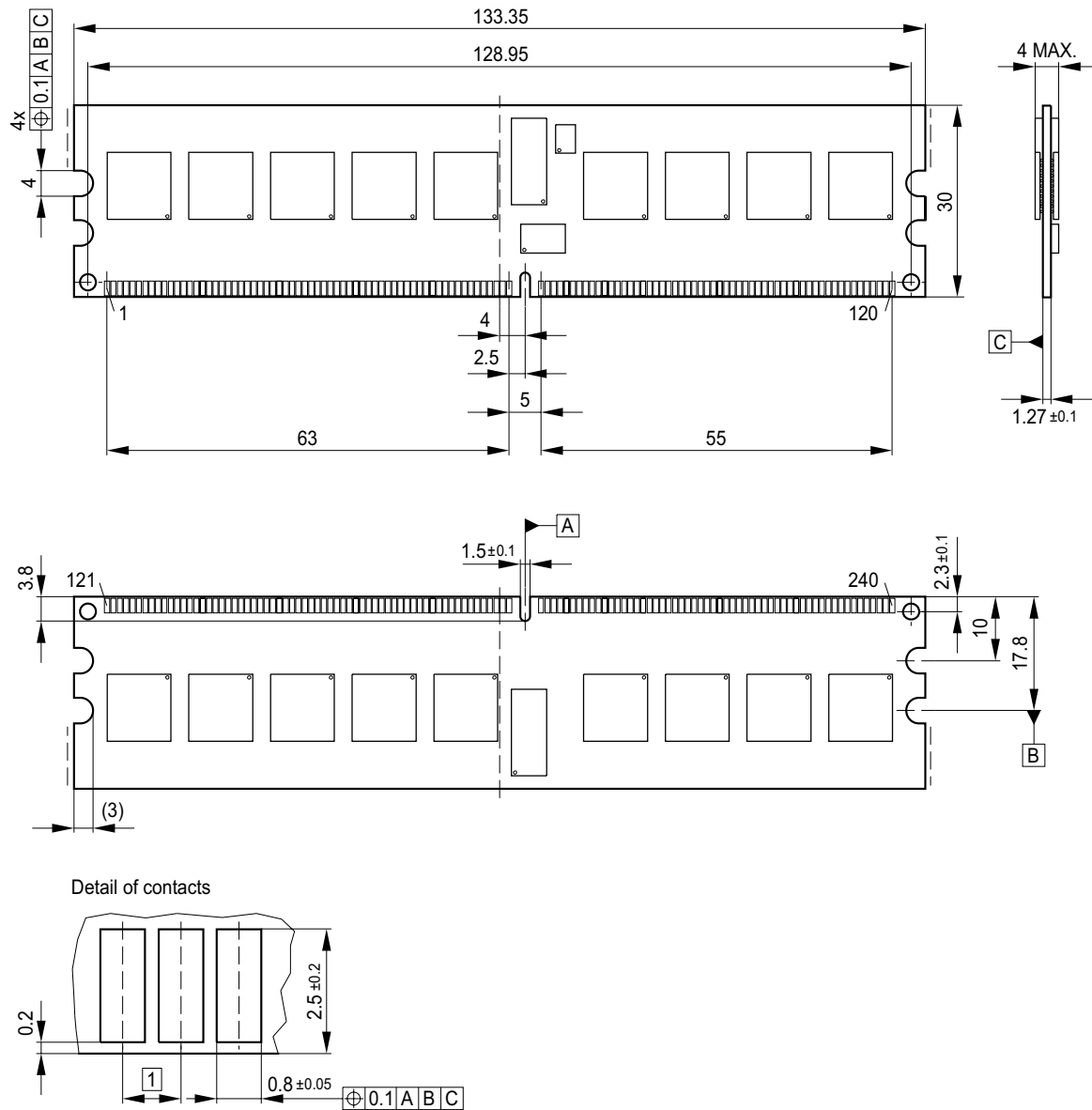
FIGURE 7 Package Outline Raw Card G L-DIM-240-12
