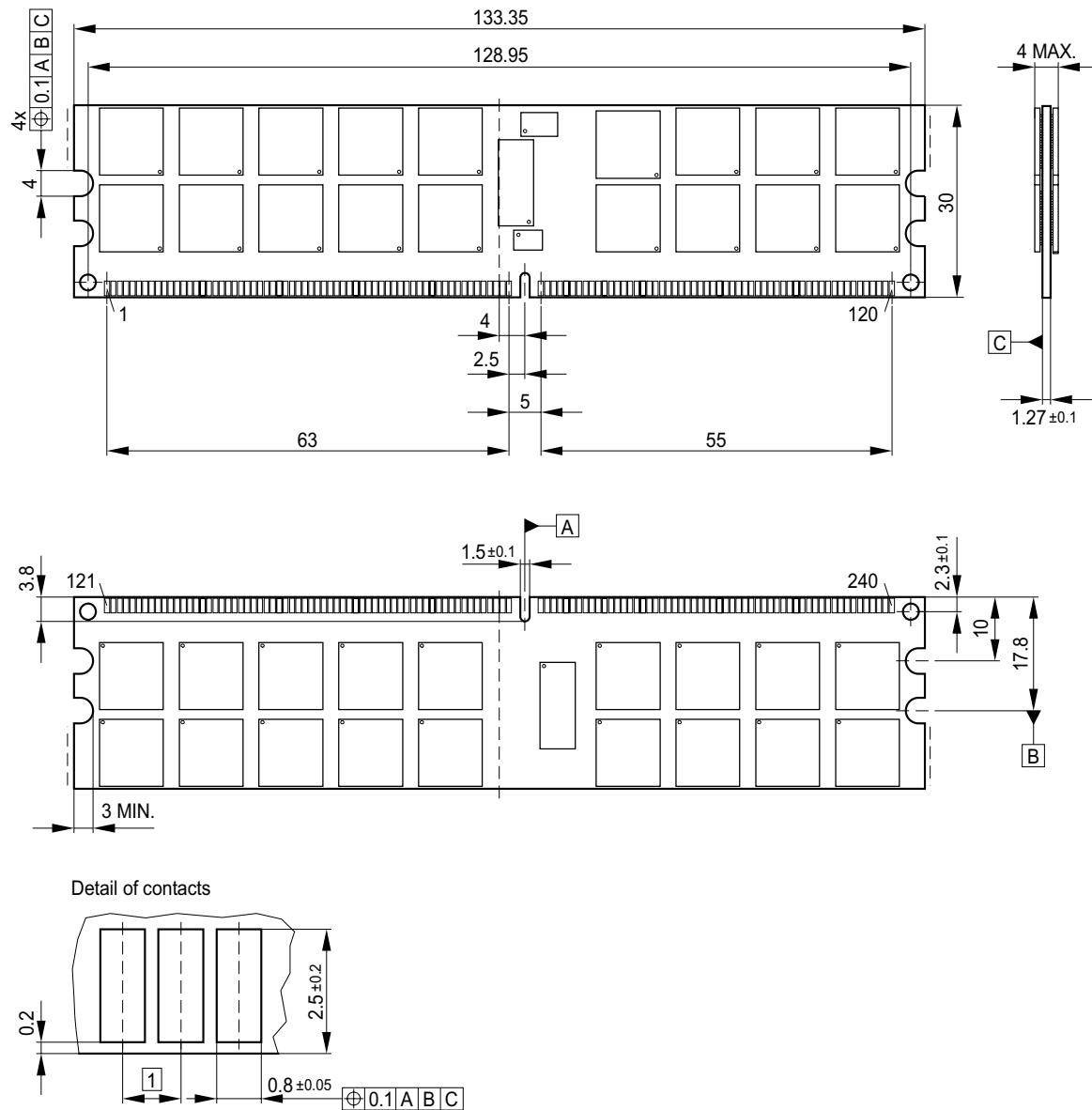
FIGURE 9 Package Outline Raw Card L L-DIM-240-48
