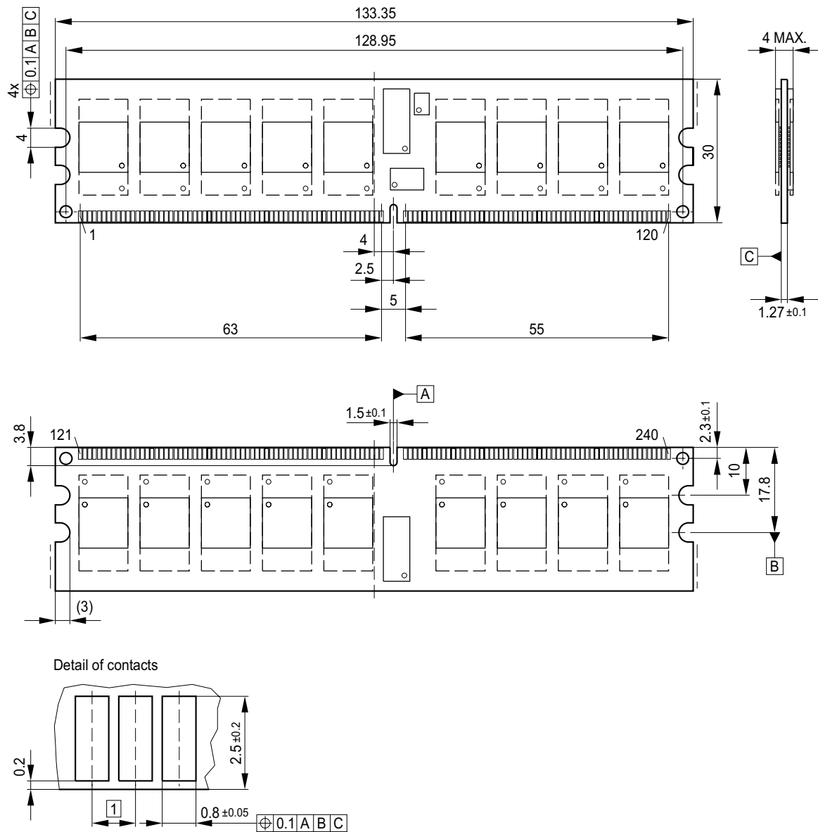
FIGURE 6 Package Outline Raw Card H L-DIM-240-13
