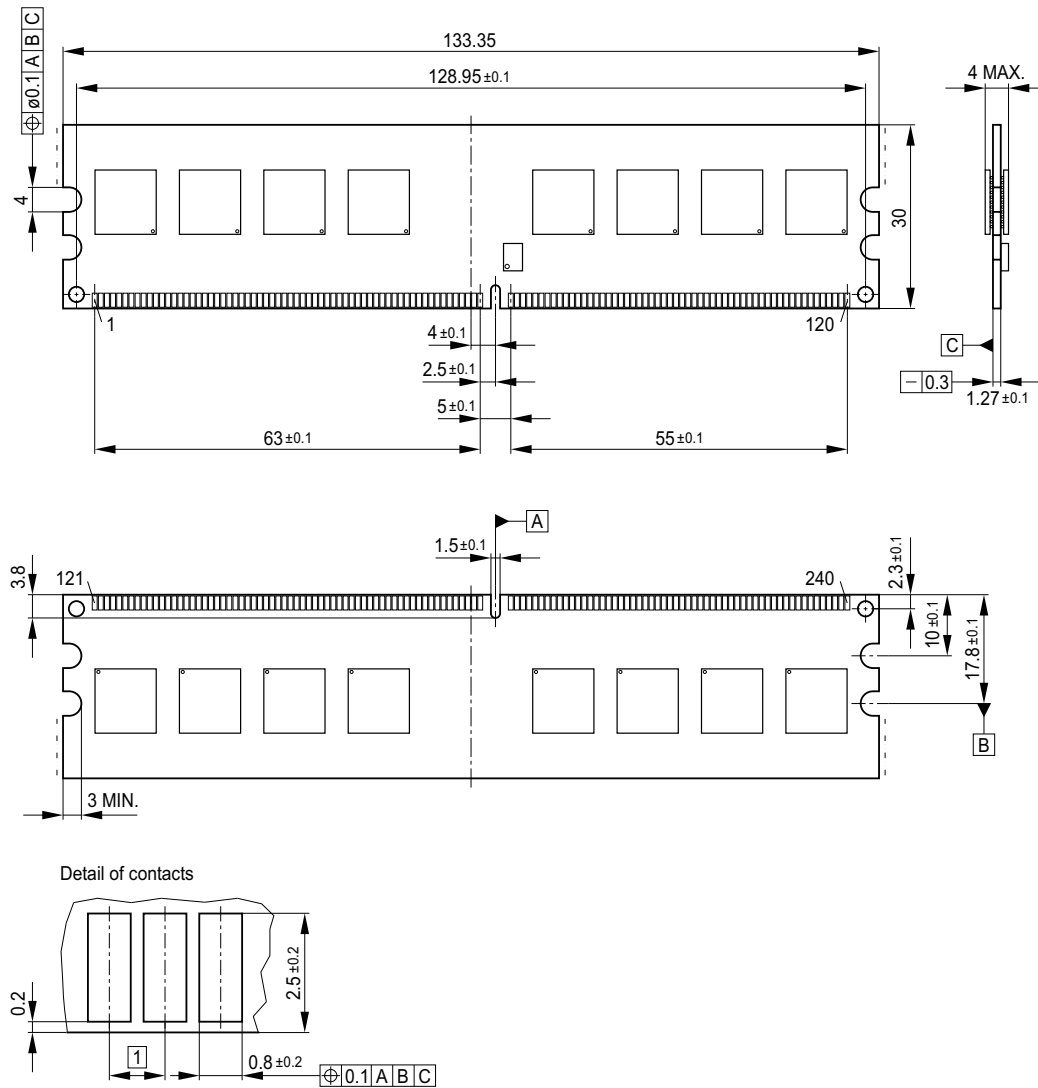
FIGURE 8 Package Outline L-DIM-240-9
