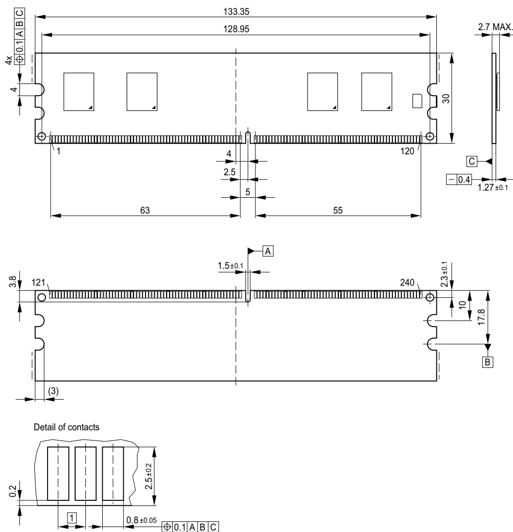
FIGURE 6 Package Outline Raw Card C L-DIM-240-3
