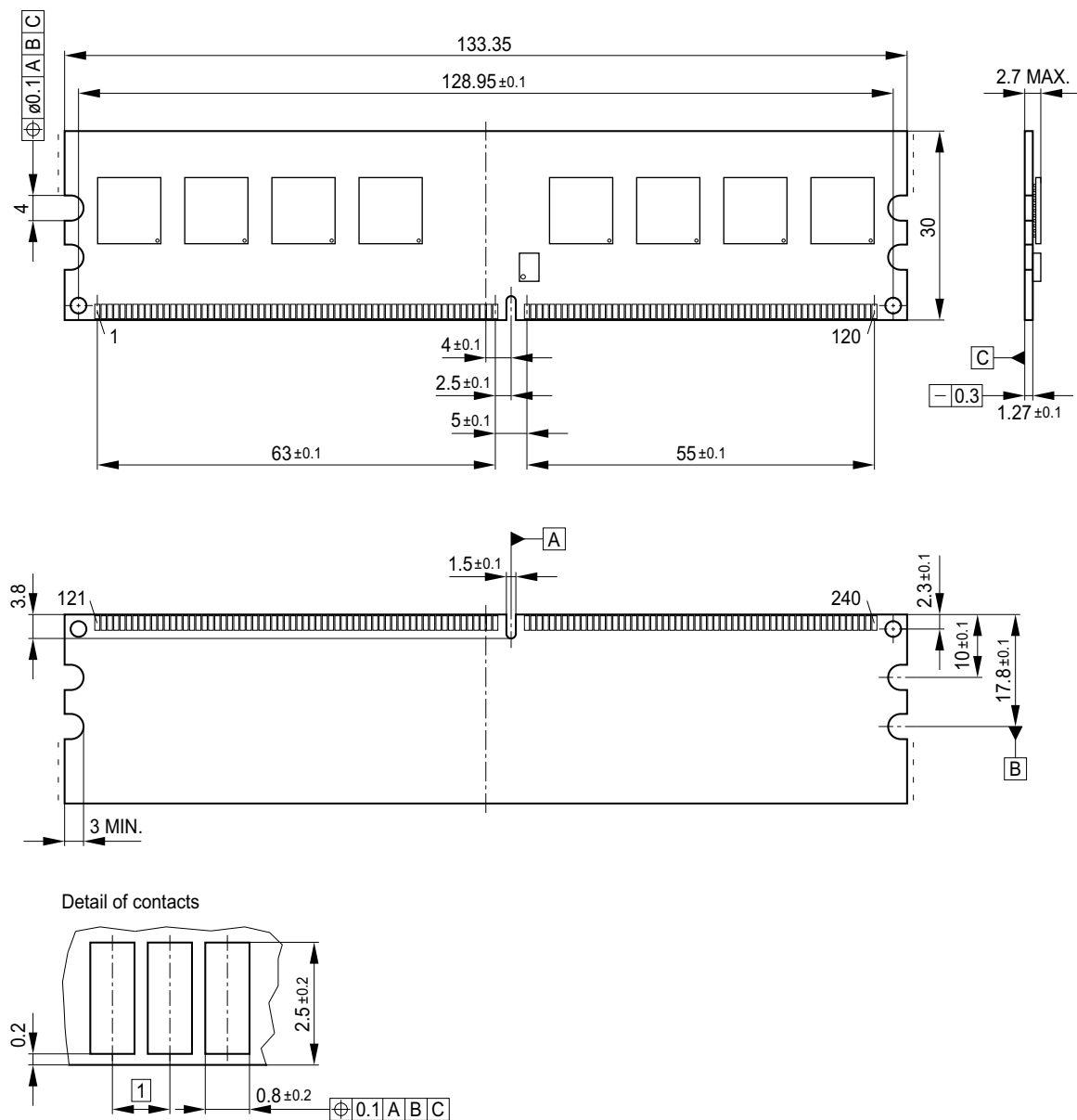
FIGURE 7 Package Outline L-DIM-240-8
