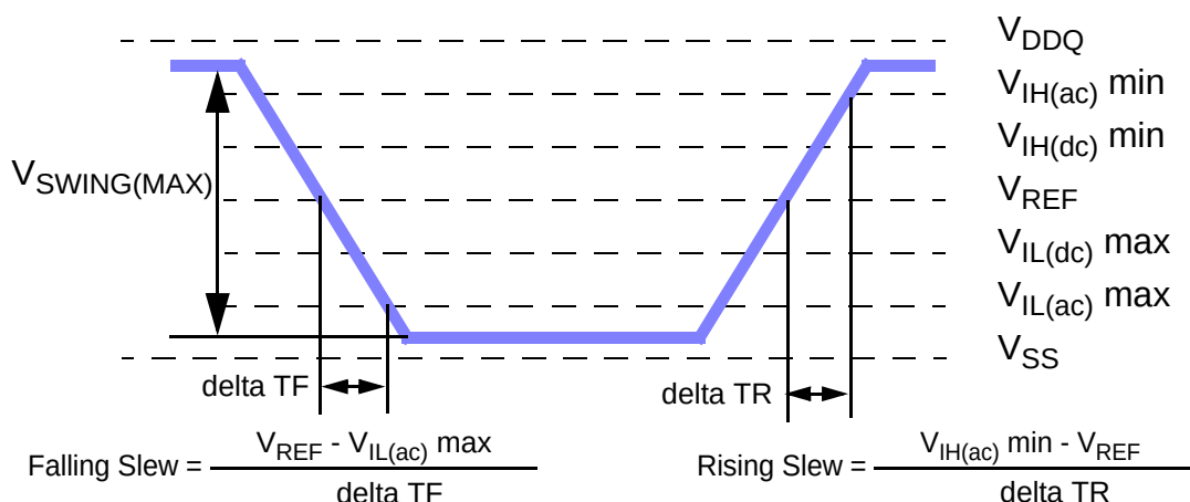
< Figure : AC Input Test Signal Waveform >
