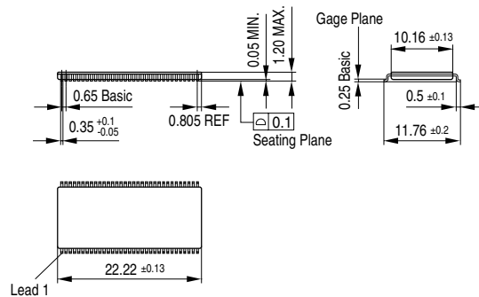
FIGURE 5 Package Outline of P(G)-TSOPII-66-1 (green/non-green)
