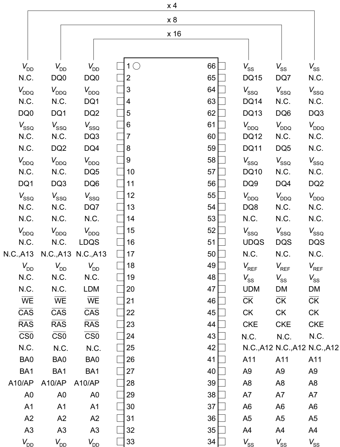
FIGURE 2 Pin Configuration P(G)-TSOPII-66
