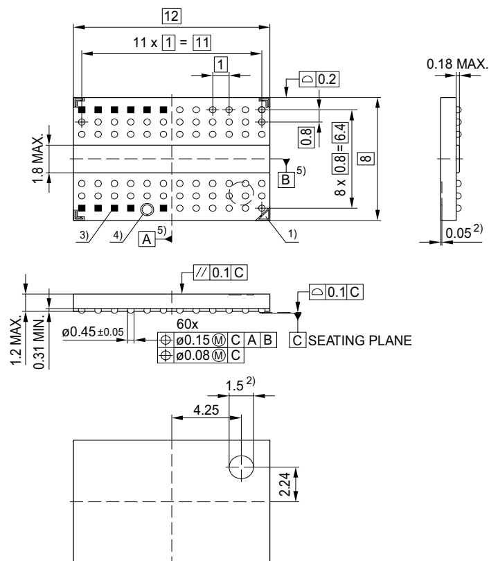
FIGURE 4 Package Outline of P-TFBGA-60-12 (non-green/green)
