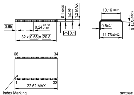
FIGURE 5 Package Outline of P-TSOP11-66-1 (non-green/green)
