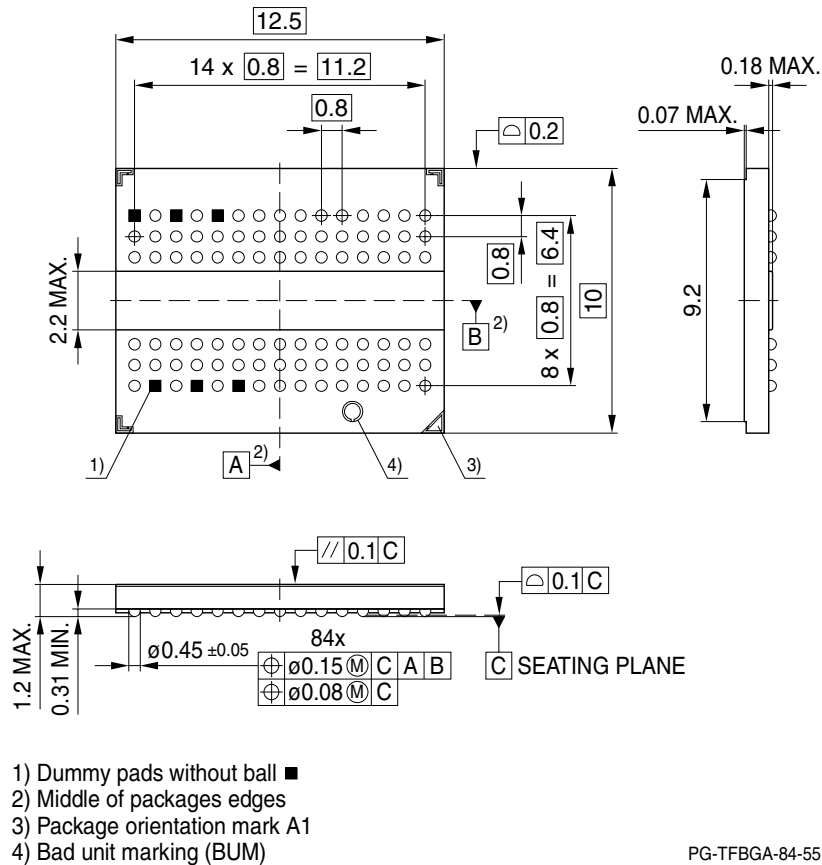
FIGURE 12 Package Outline P(G)-TFBGA-84
