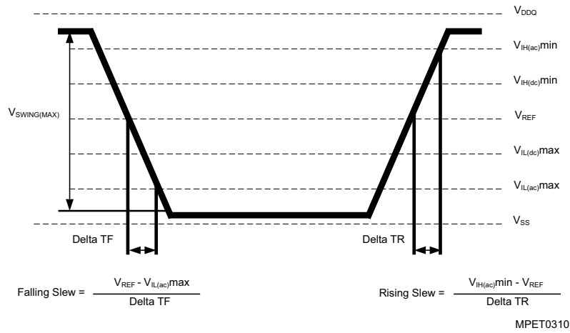
FIGURE 4 Single-ended AC Input Test Conditions Diagram
