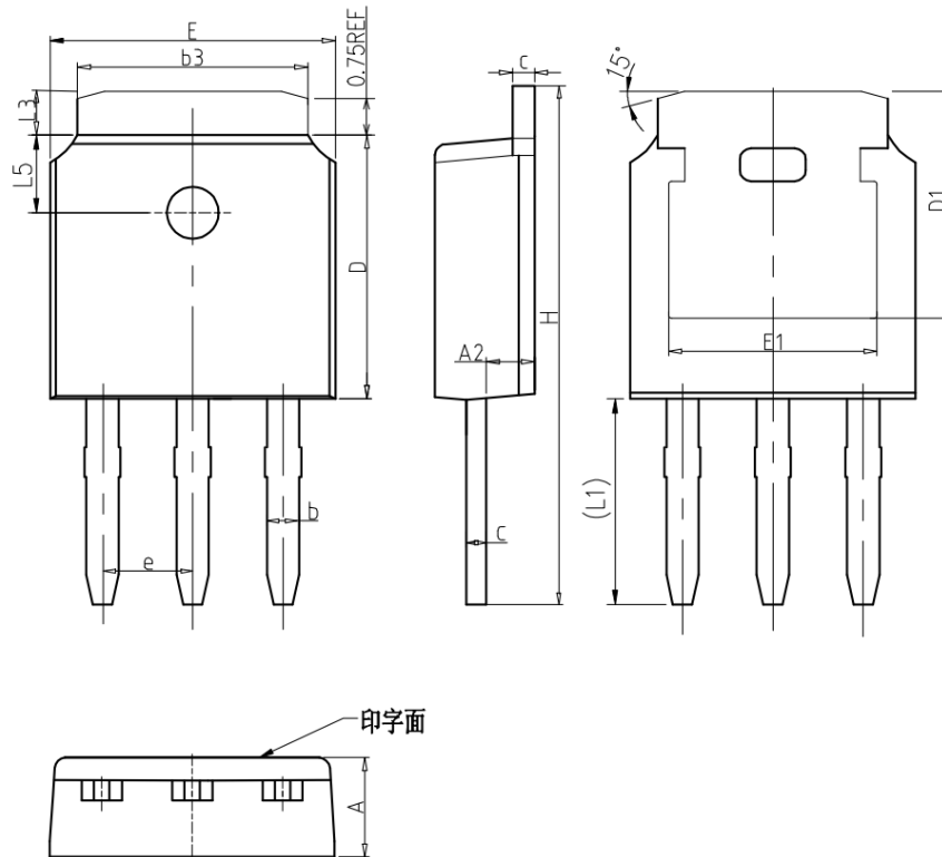
COMMON DIMENSIONS
