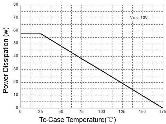
Figure 1: Power Dissipation
