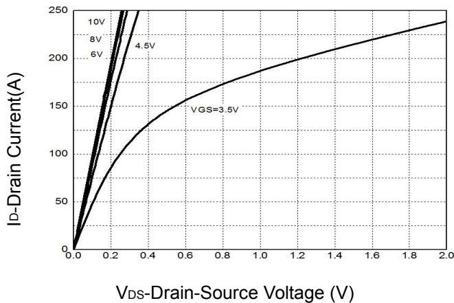
Figure 5: Output Characteristics
