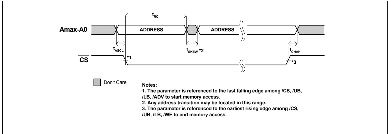
Figure 19 Timing Diagram of Address Skew
