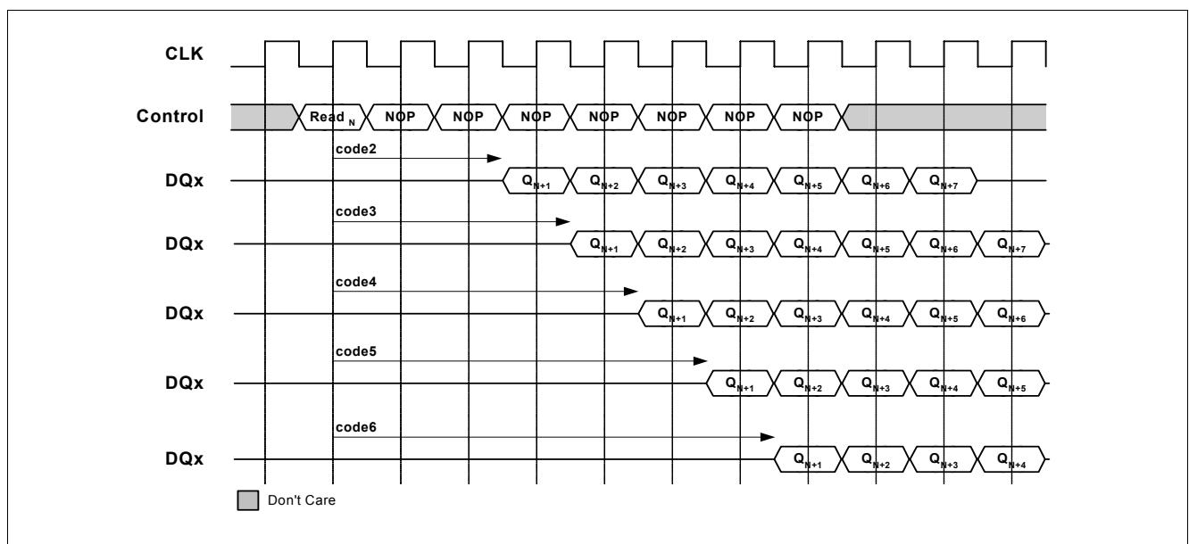
Figure 14 Latency Code - Functional Diagram
