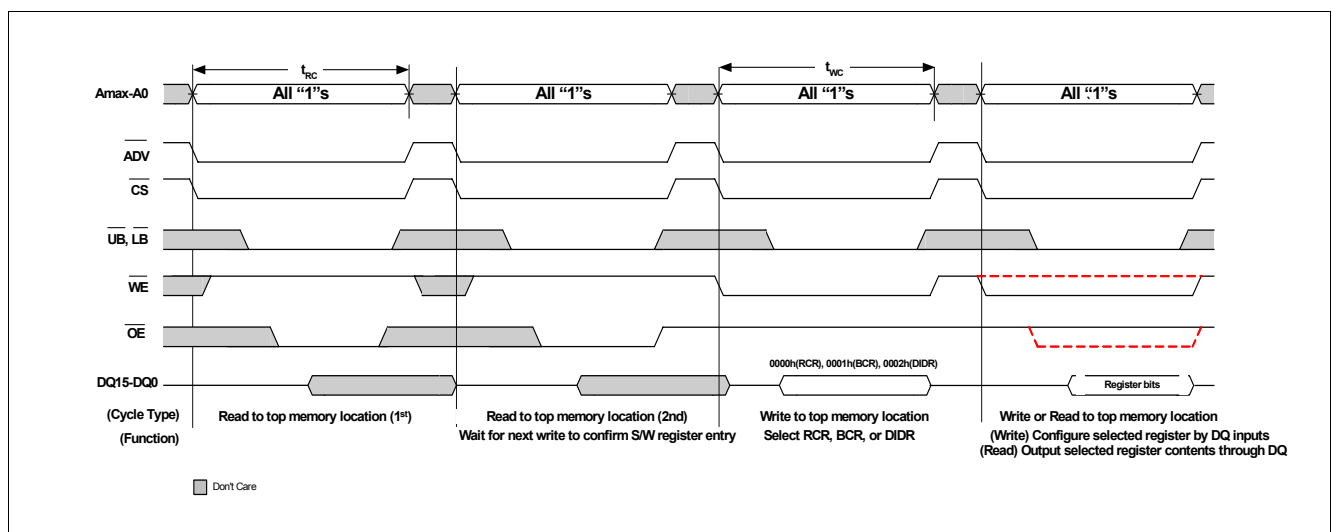
Figure 41 S/W Register Entry timing (Address input = 7FFFF H )
