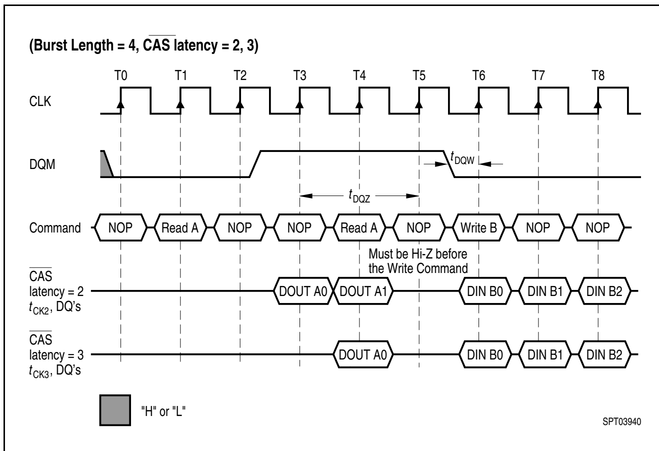
Figure 10 Non-Minimum Read to Write Interval
