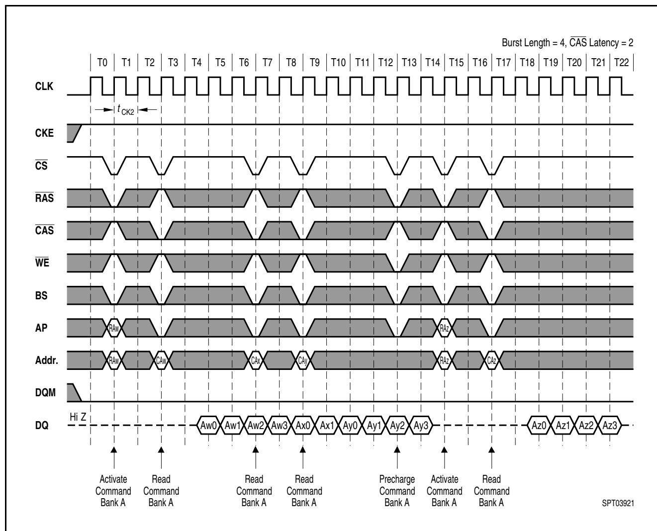
Figure 27 CAS Latency = 2
