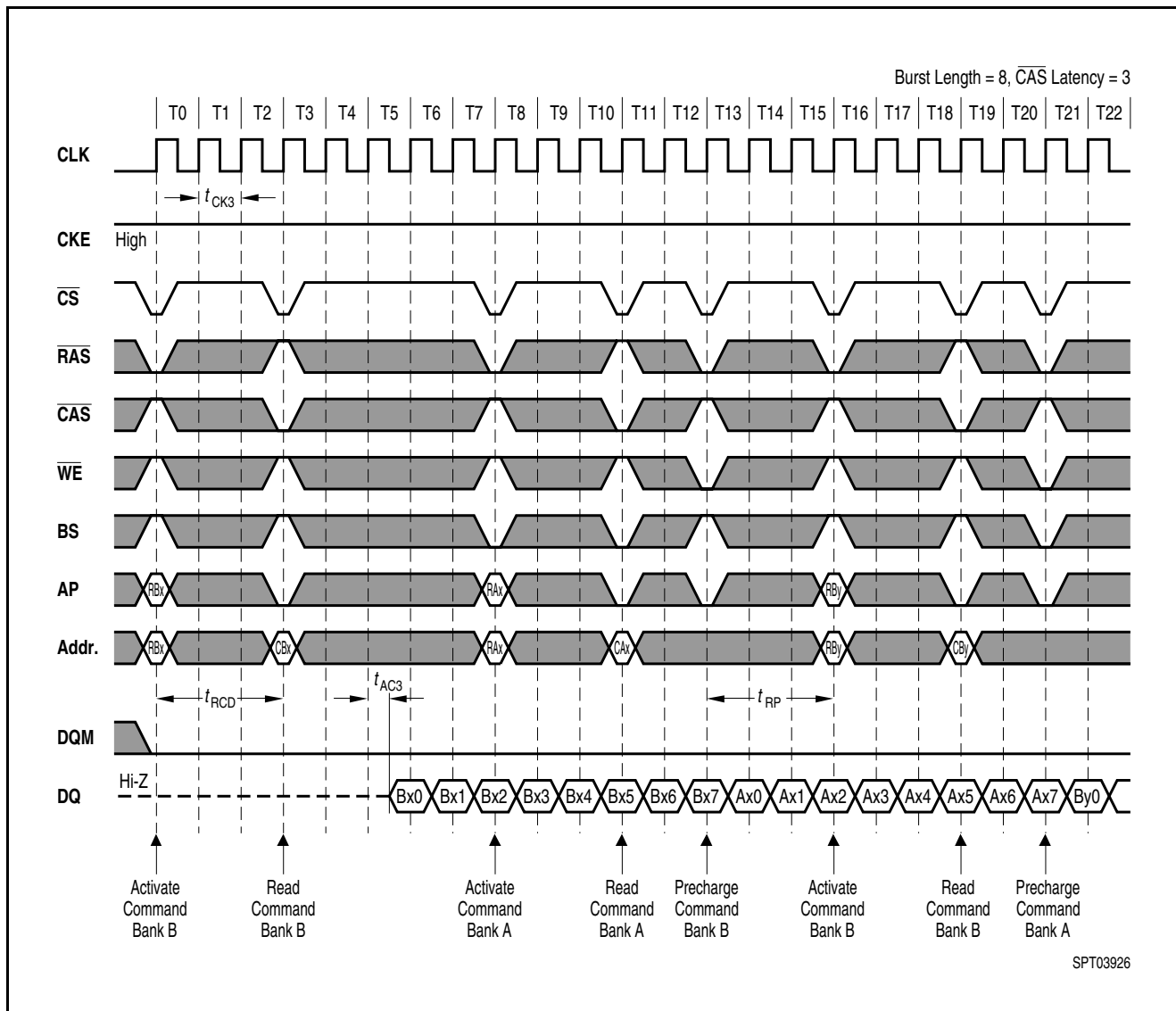
Figure 32 CAS Latency = 3
