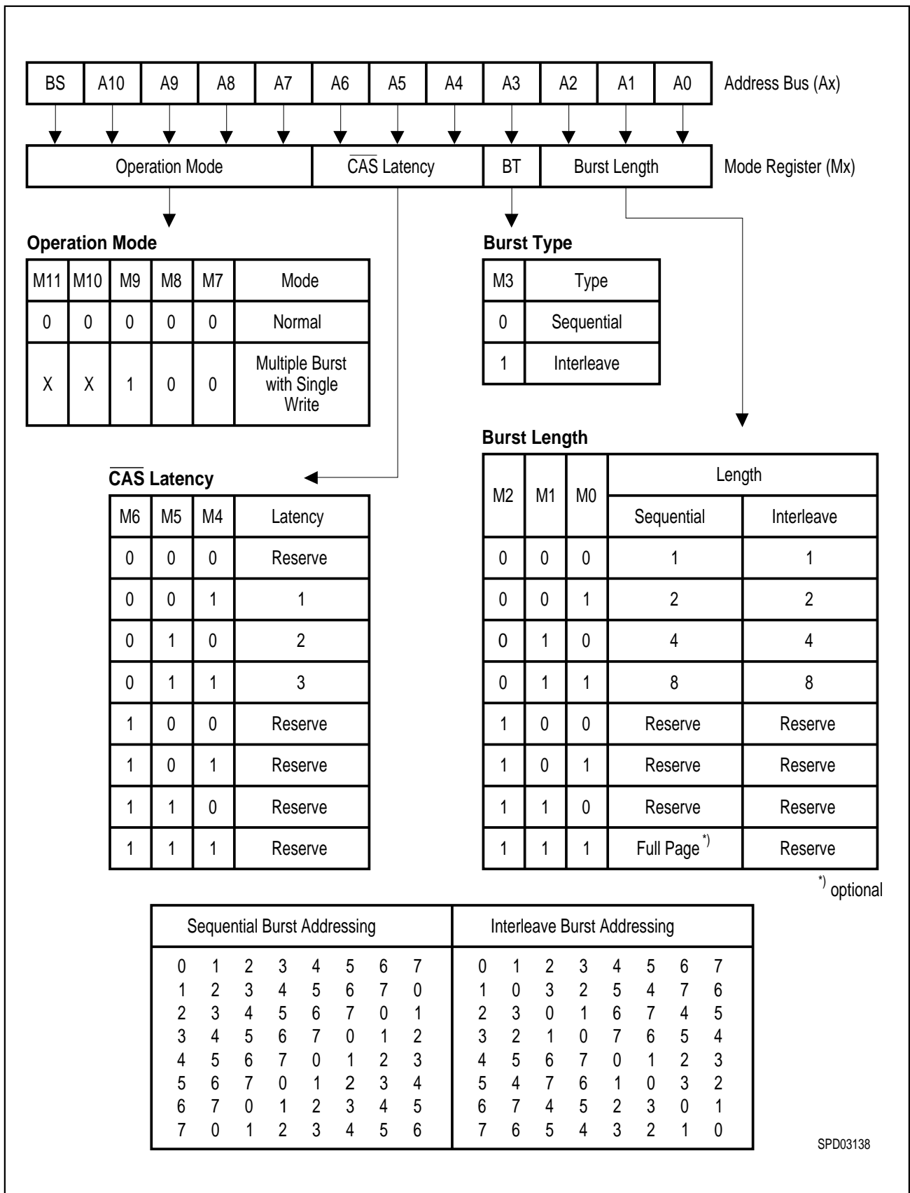
Address Input for Mode Set (Mode Register Operation)
