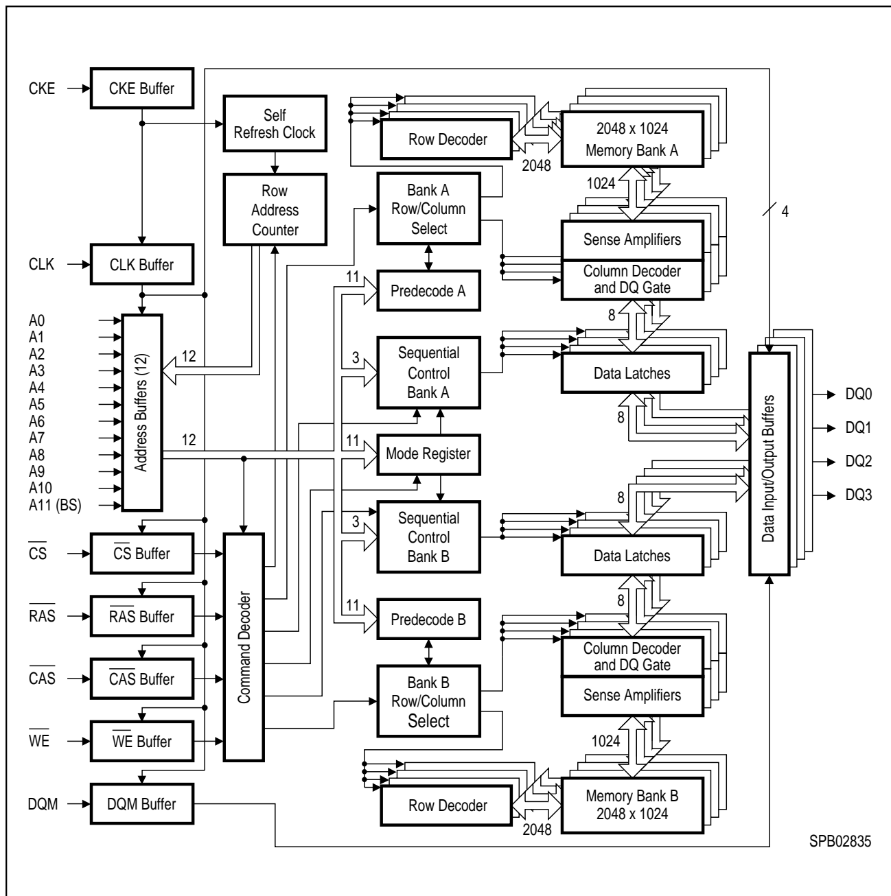
Block Diagram for HYB 39S16400CT (2 banks x 2 M x 4 SDRAM)
