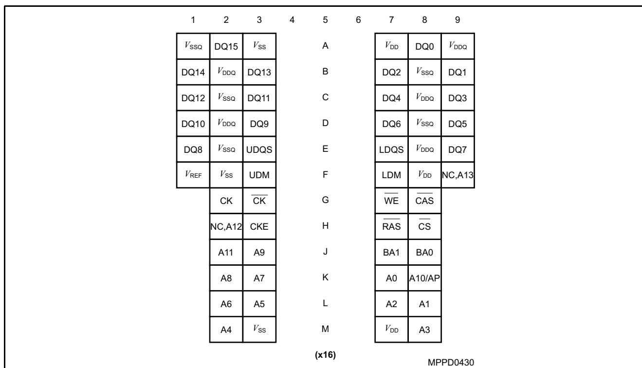
Figure 2 Pin Configuration PG-TFBGA-60 (top view) for \times 16 , see the balls throught the package
