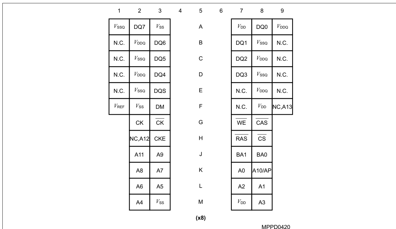
Figure 1 Pin Configuration PG-TFBGA-60 (top view) for \times 8 , see the balls throught the package
