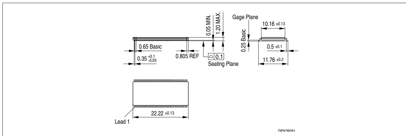
Figure 55 Package Outline of PG-TSOPII-66-1 (green/non-green)
