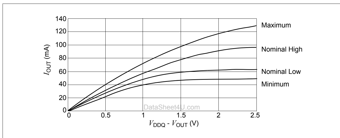
Figure 34 Normal Strength Pull-down Characteristics
