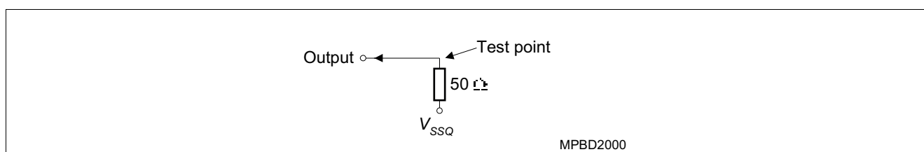
Figure 53 Pulldown slew rate test load
