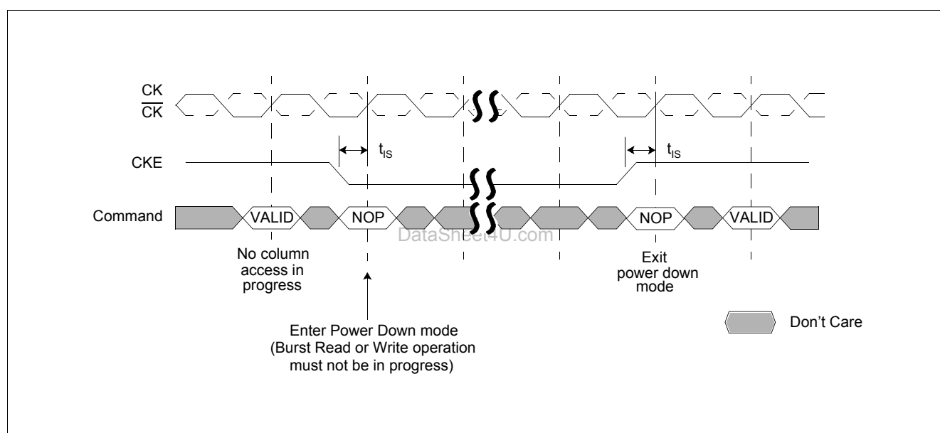
Figure 31 Power Down
