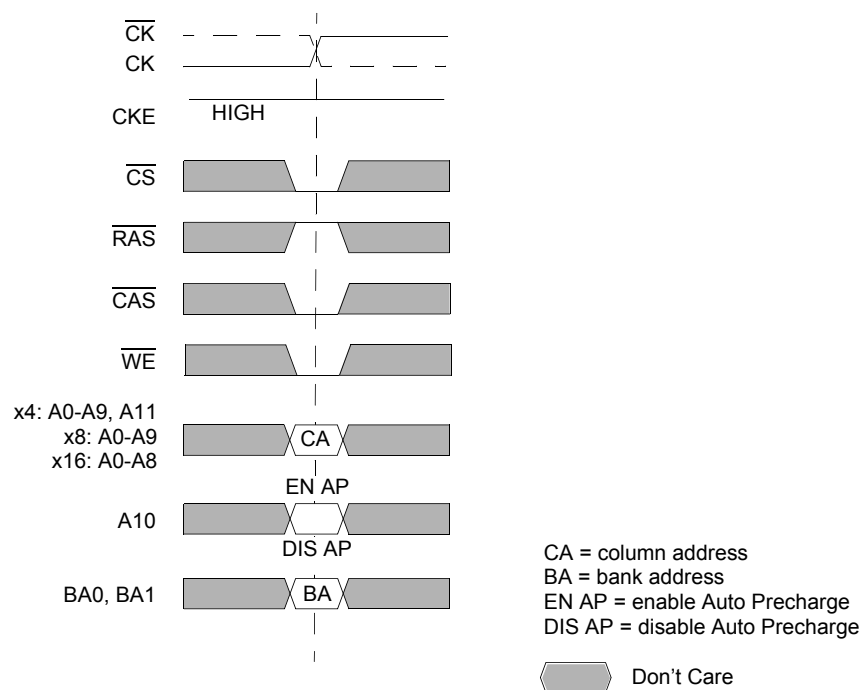
Figure 17 Write Command
