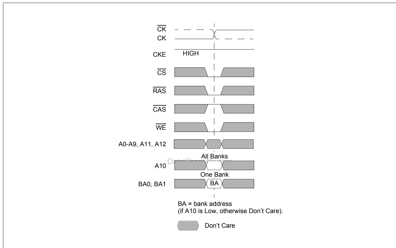
Figure 30 Precharge Command
