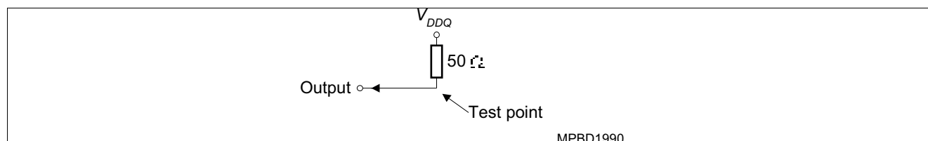
Figure 52 Pullup slew rate test load
