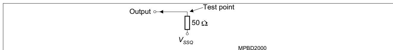
Figure 53 Pulldown slew rate test load
