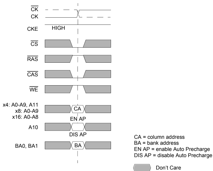
Figure 9 Read Command
