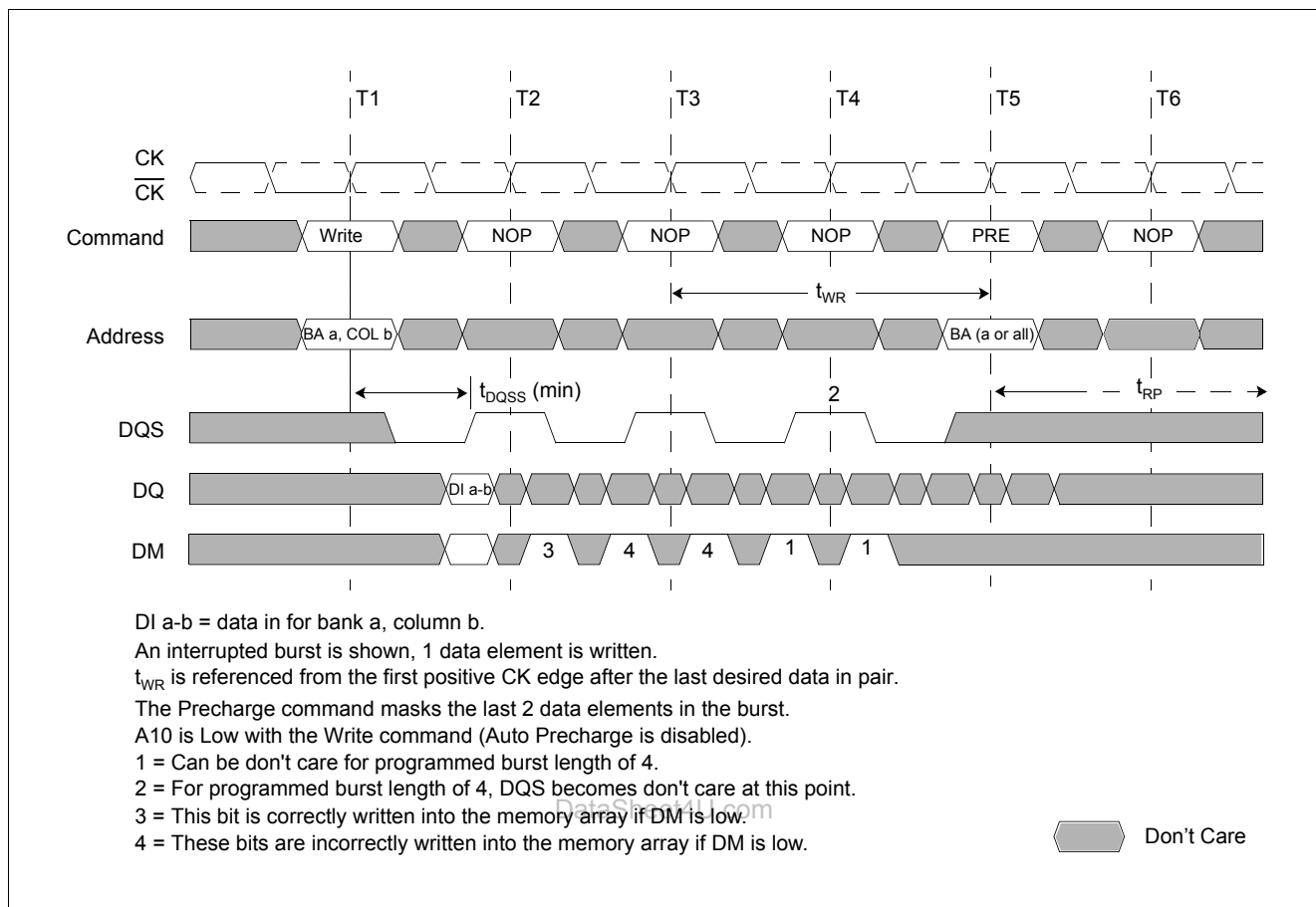
Figure 28 Write to Precharge: Minimum DQSS, Odd Number of Data (1-bit Write), Interrupting (BL 4 or 8)
