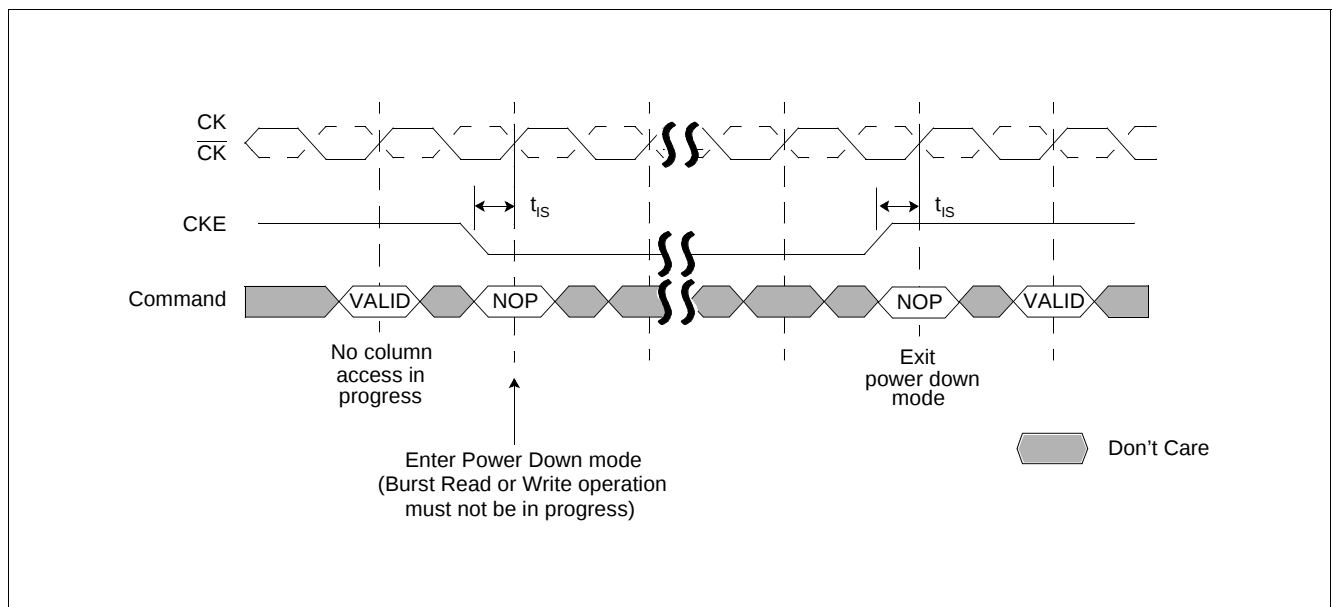
Figure 26 Power Down
