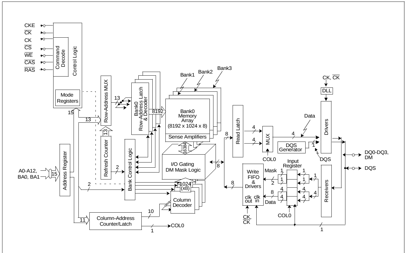
Figure 3 Block Diagram (64 Mbit × 4)
