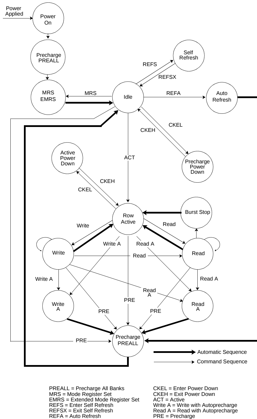
Figure 27 Simplified State Diagram
