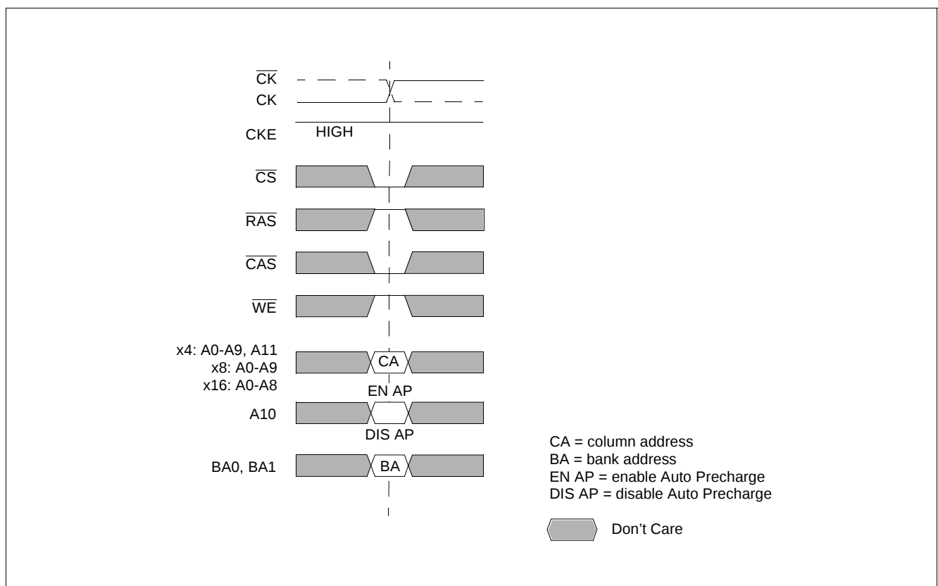
Figure 4 Read Command
