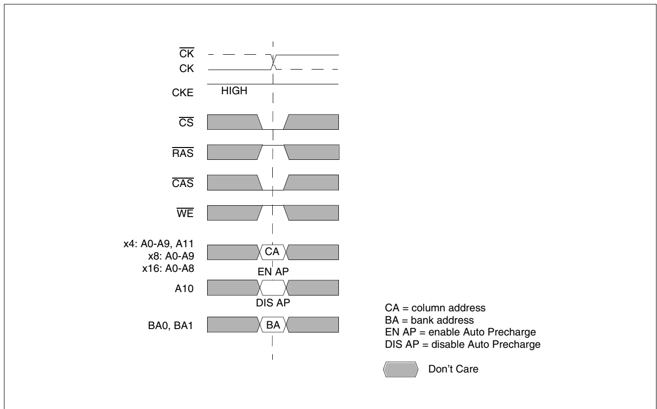
Figure 9 Read Command
