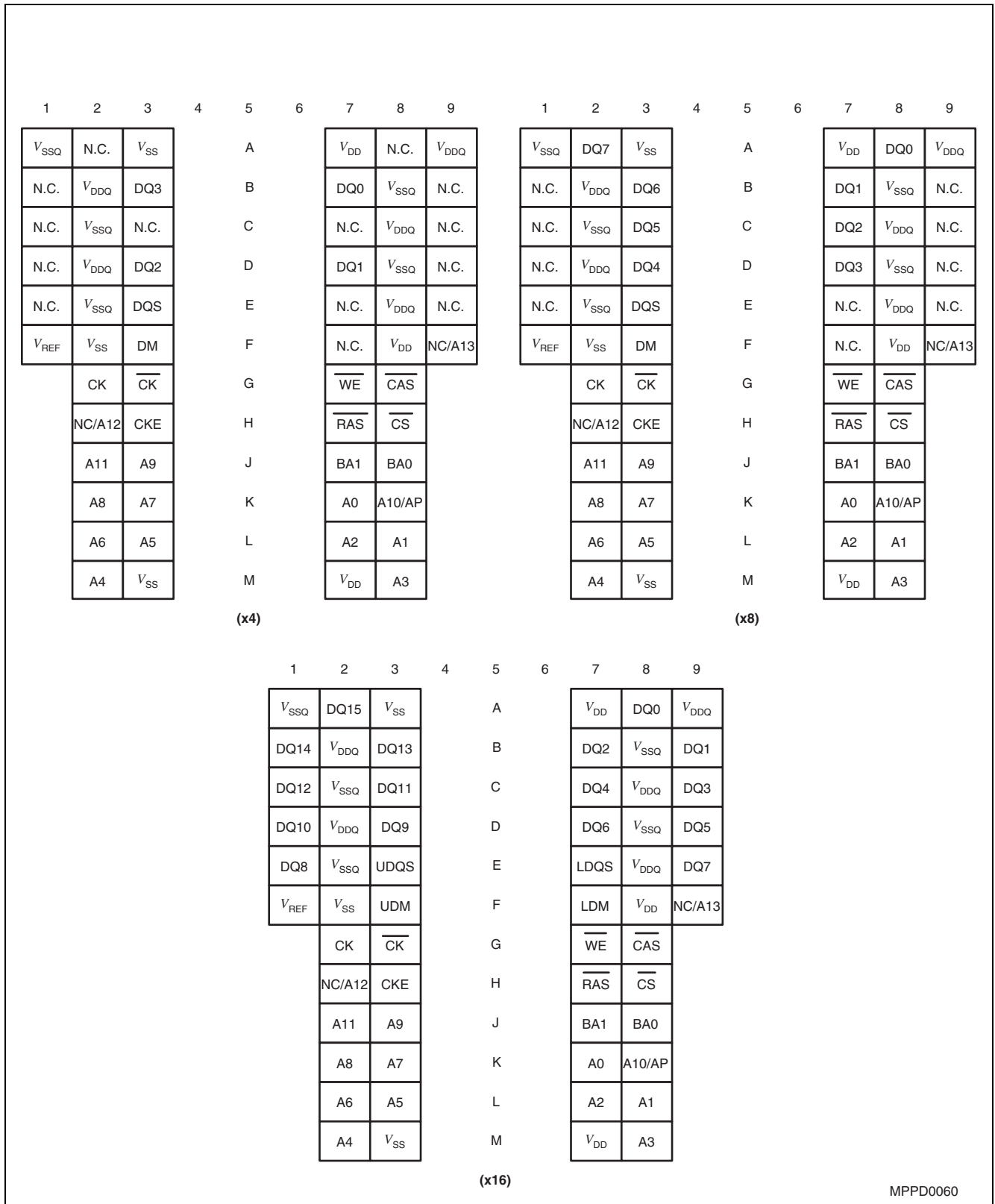
Figure 1 Pin Configuration P-TFBGA-60-9 Top View, see the balls throught the package
