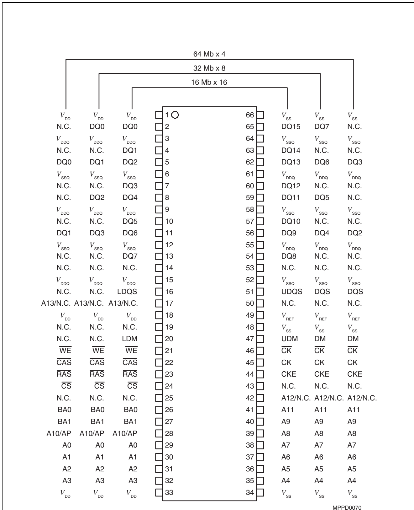
Figure 2 Pin Configuration P-TSOP16-1
