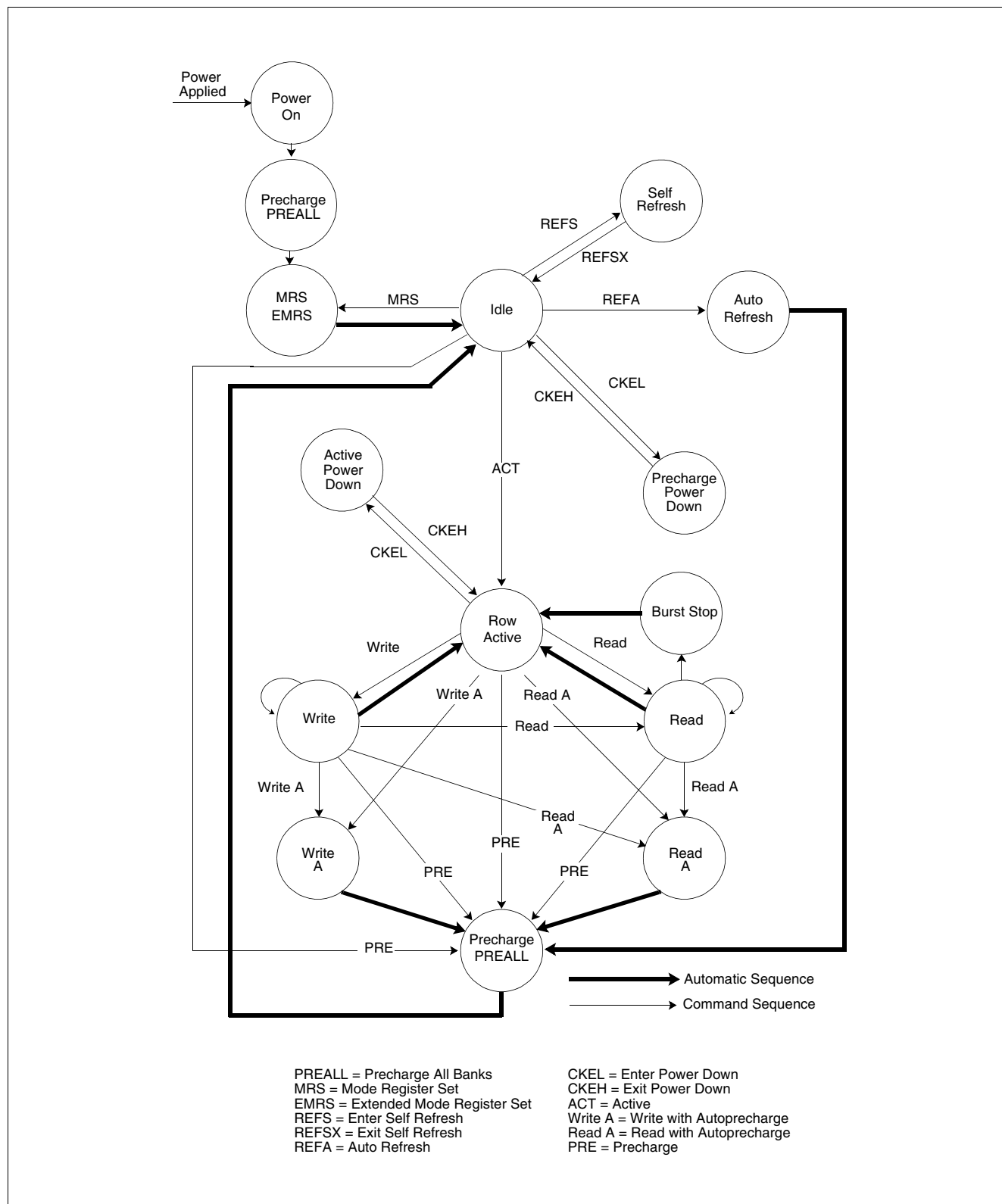
Figure 32 Simplified State Diagram
