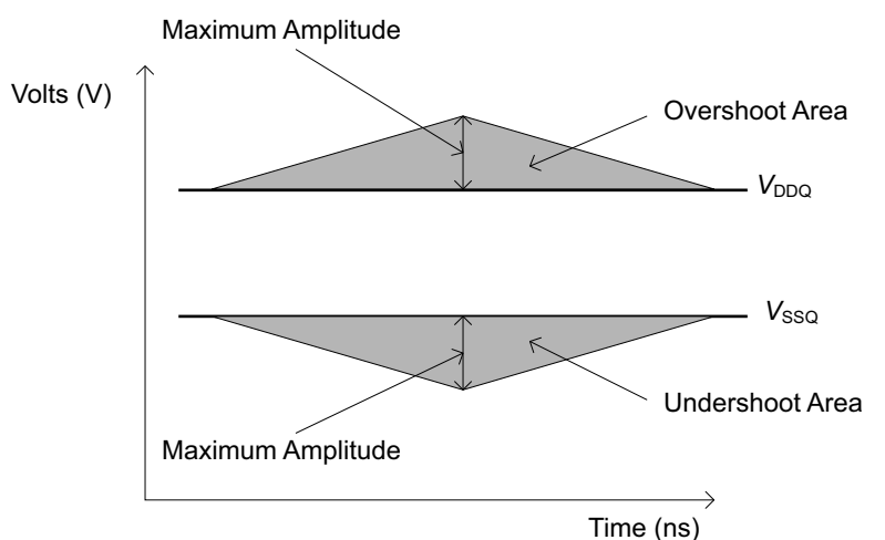
FIGURE 6 AC Overshoot / Undershoot Diagram for Clock, Data, Strobe and Mask Pins
