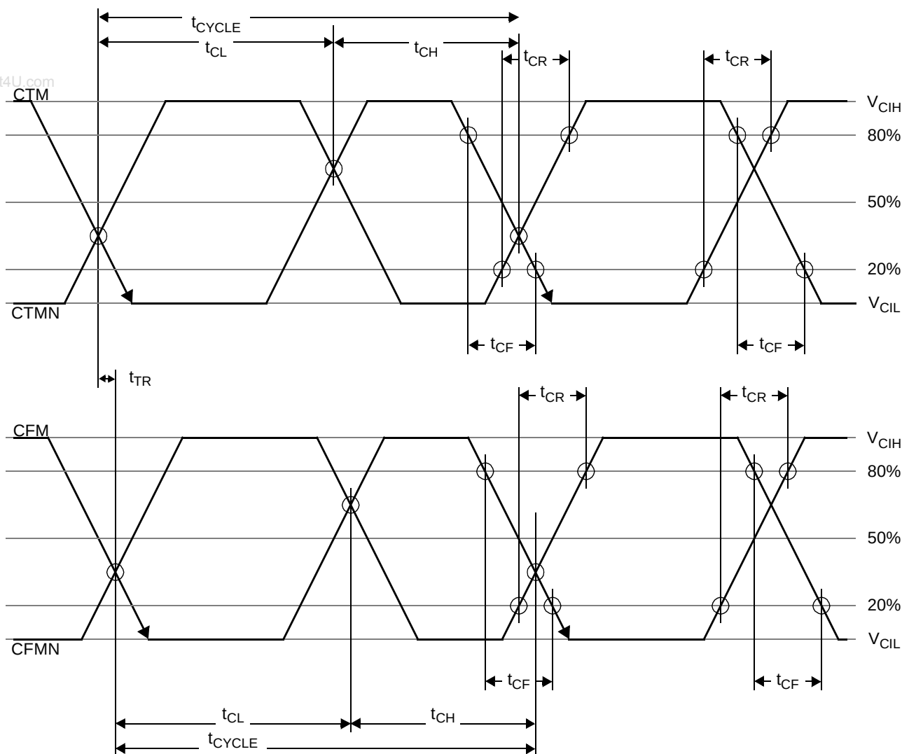
Figure 54: RSL Timing - Clock Signals
