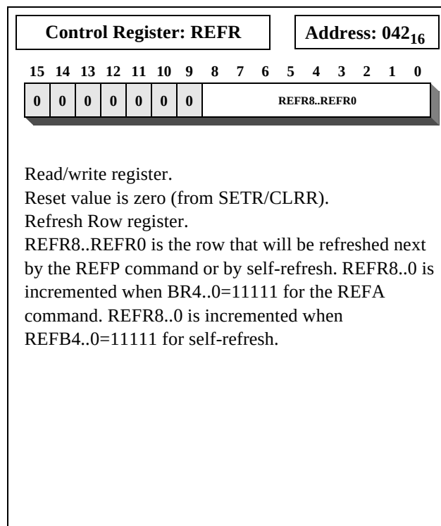
Figure 34: REFR Register
