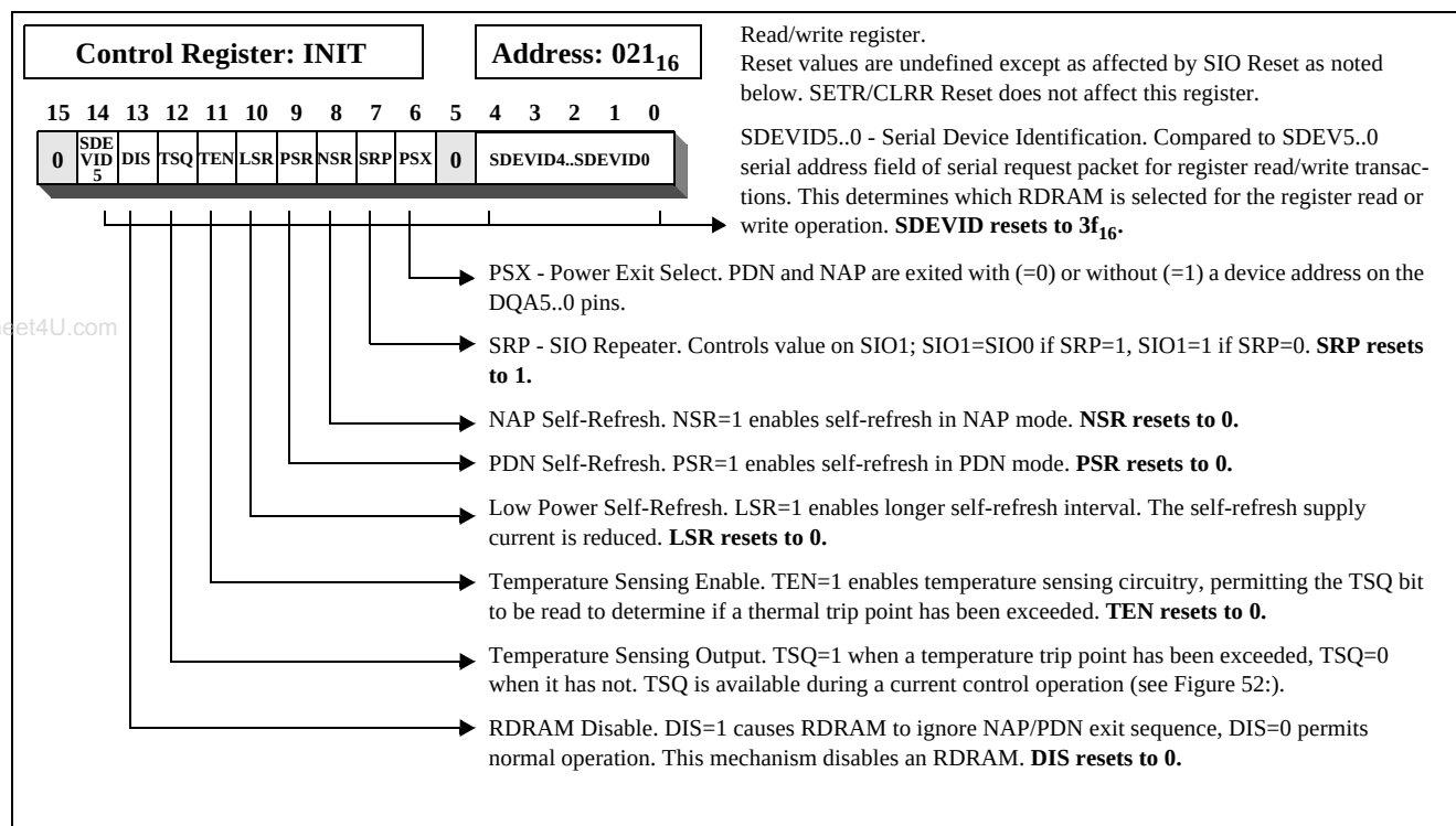
Figure 27: INIT Register
