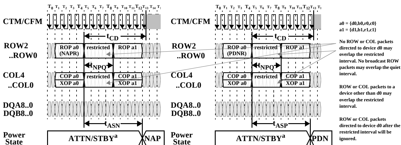
Figure 47: NAP Entry (left) and PDN Entry (right)
