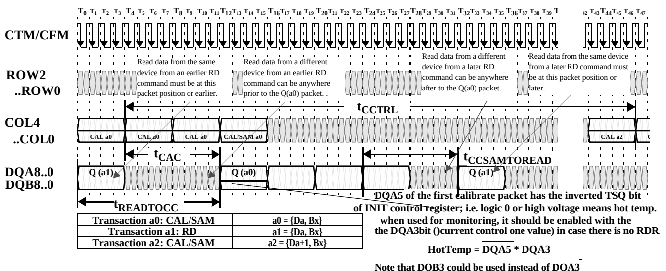
Figure 52: Current Control CAL/SAM Transaction Example
