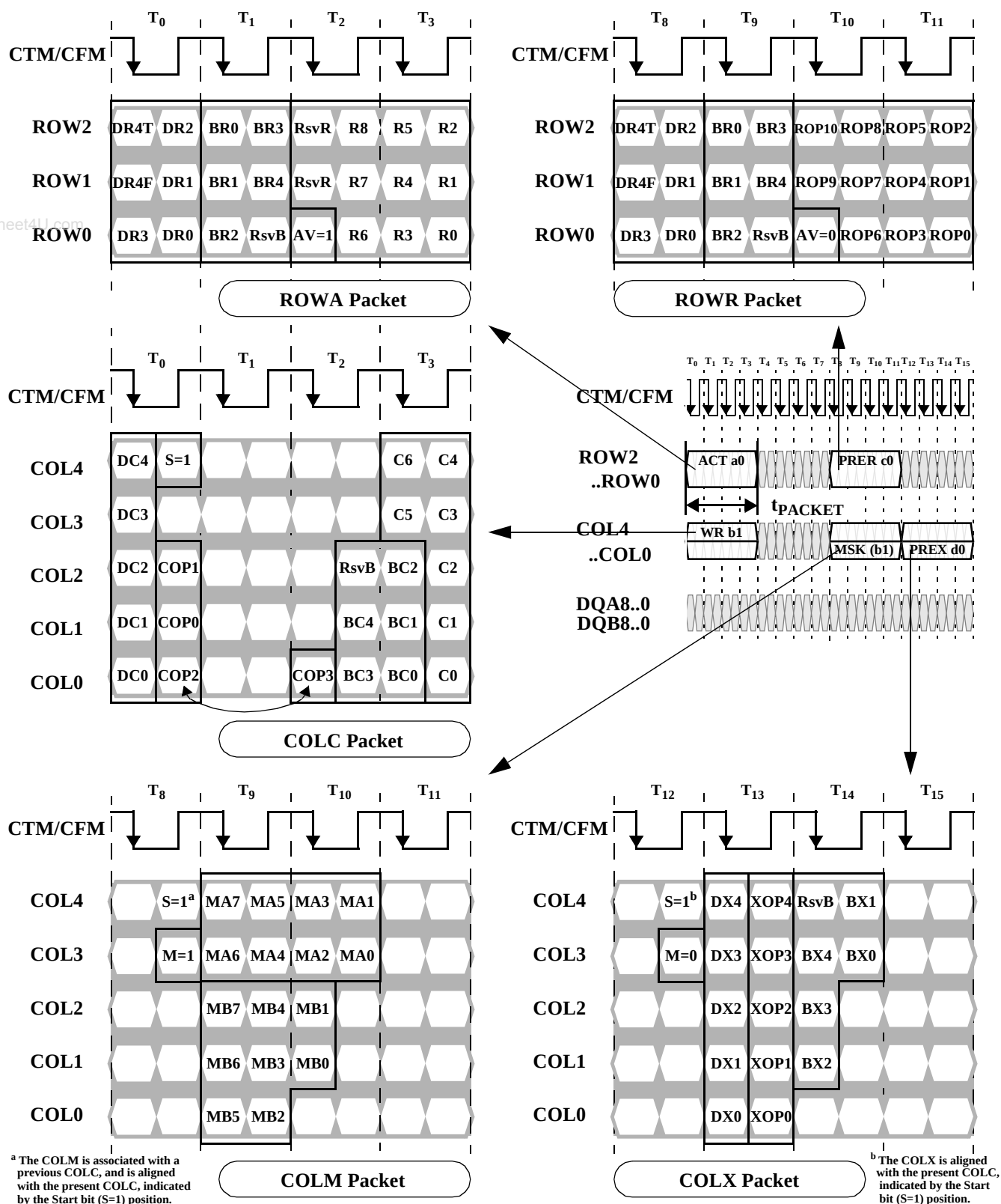
Figure 3: Packet Formats
