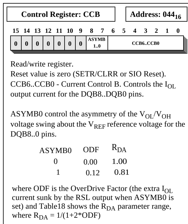
Figure 35: CCB Register
