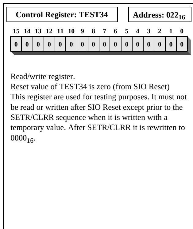
Figure 30: TEST Register
