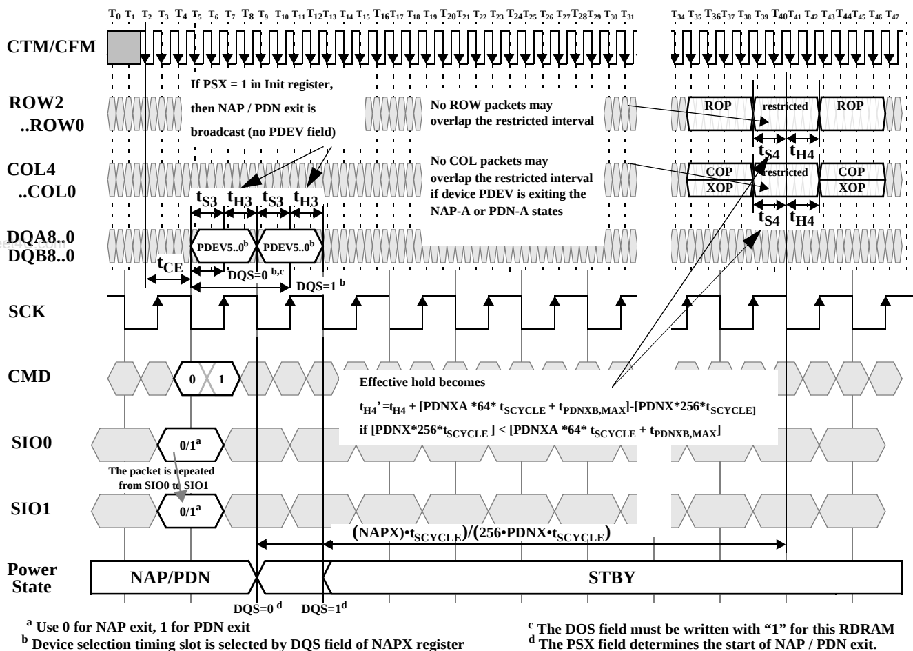
Figure 48: NAP and PDN Exit
