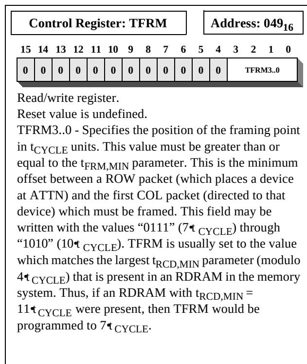
Figure 40: TFRM Register
