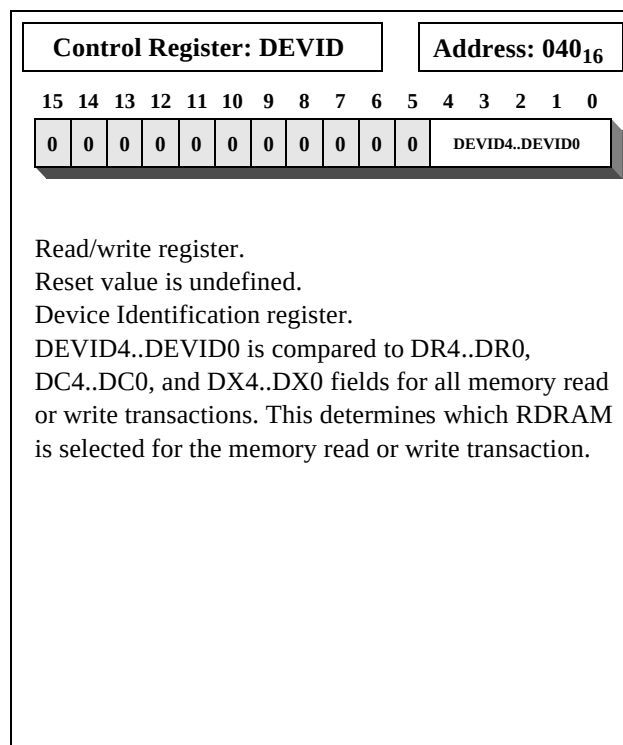
Figure 31: DEVID Register
