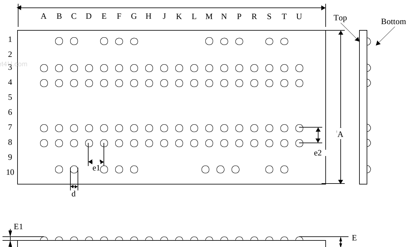
Figure 61: Center-Bonded uBGA Package
