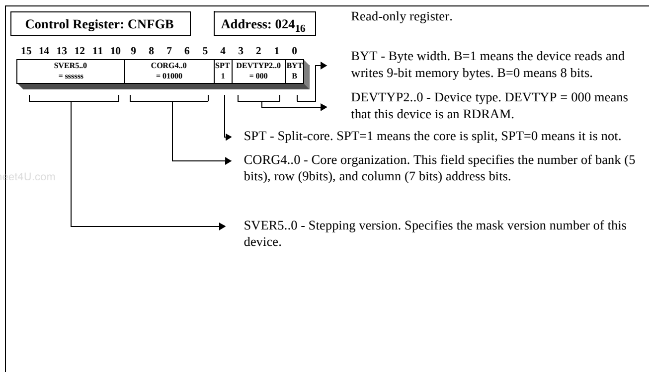
Figure 29: CNFGB Register
