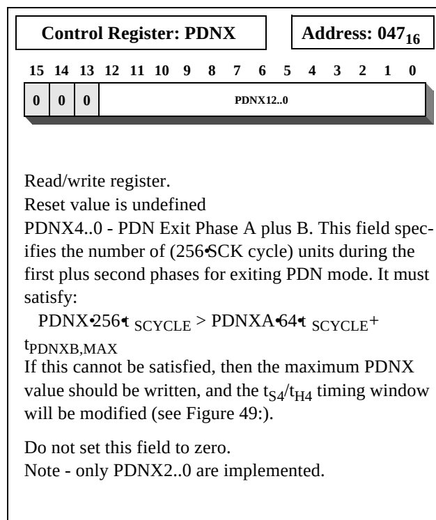
Figure 38: PDNX Register
