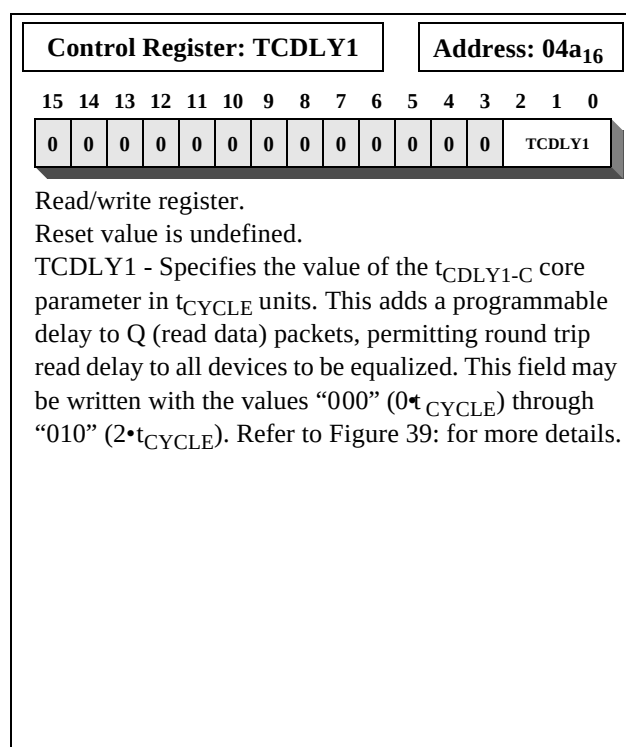
Figure 41: TRDLY Register
