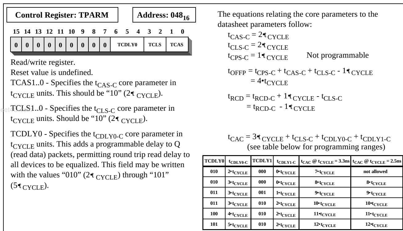
Figure 39: TPARM Register
