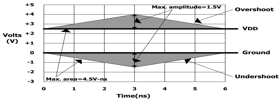
Figure 1: Address and Control AC Overshoot and Undershoot Definitio
