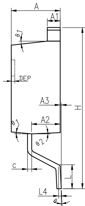
COMMON DIMENSIONS
