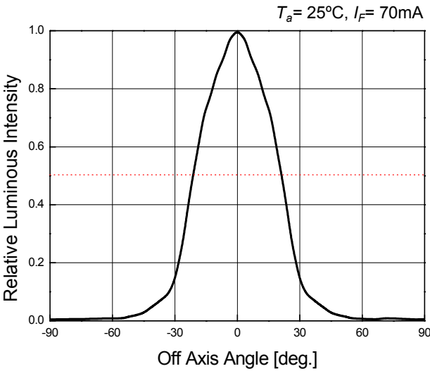
Directivity
