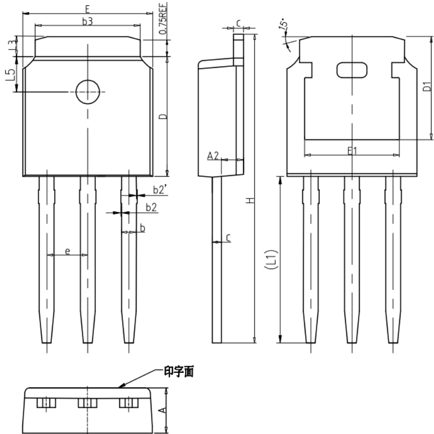
COMMON DIMENSIONS
