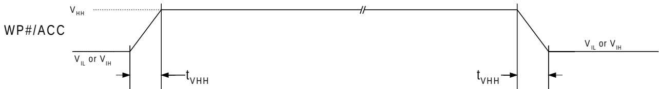
Figure 26. Accelerated Programming Timings
