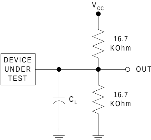
Figure 13. Test Setup
