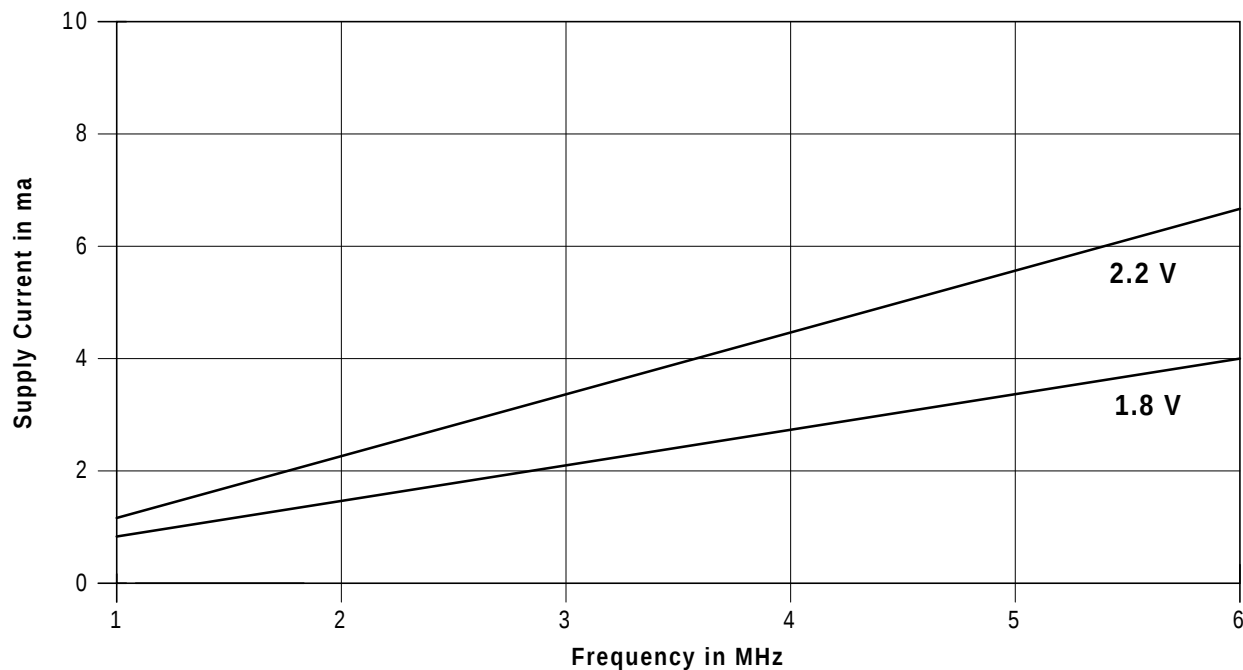
Figure 12. Typical I_{CC1} Current vs. Frequency
