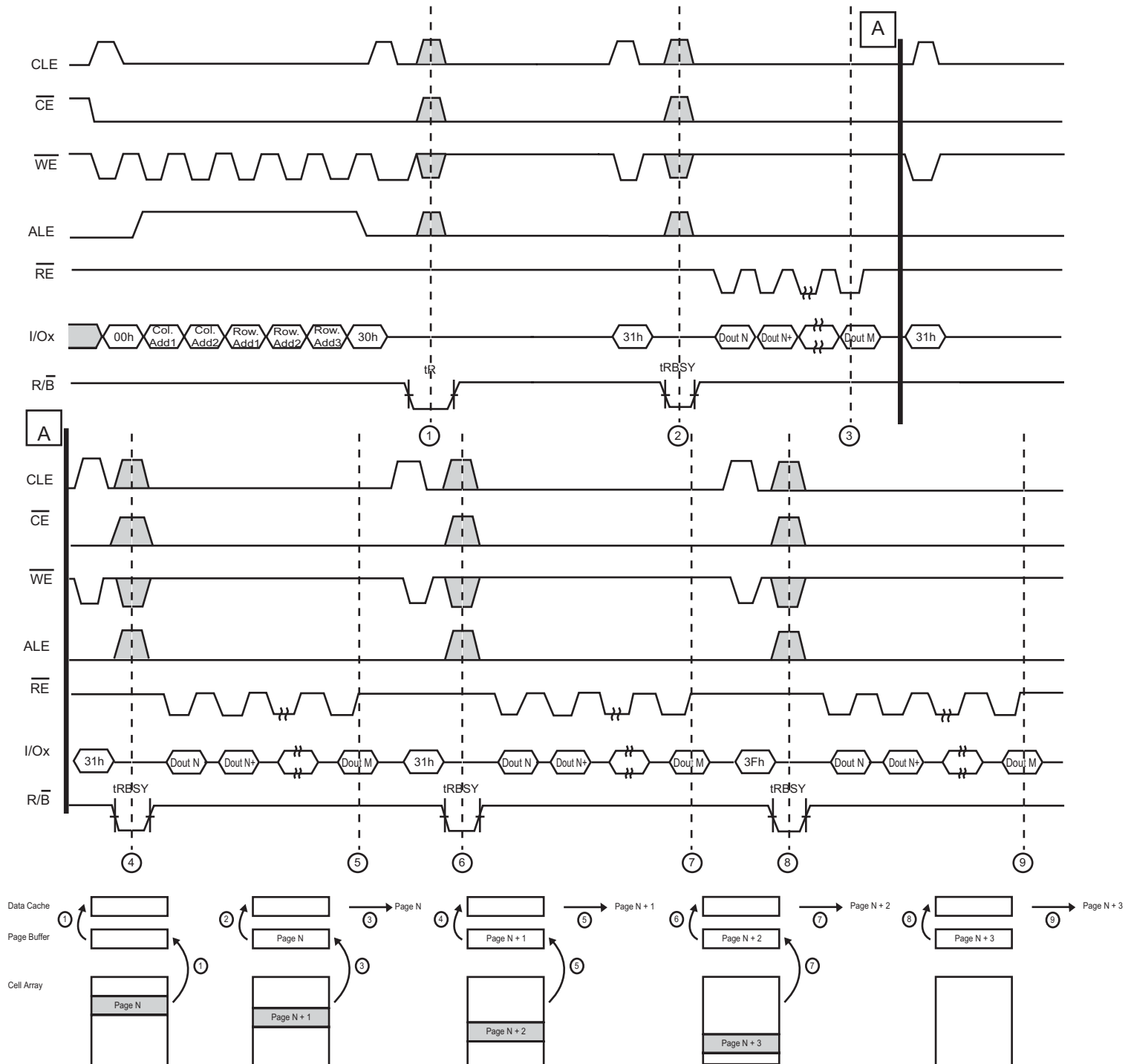
Figure 15: Read Operation with Read Cache
