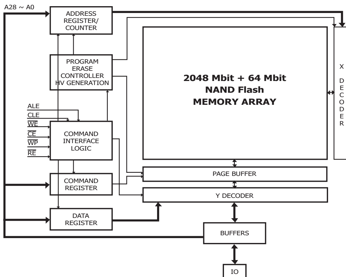
Figure 5: Block Diagram
