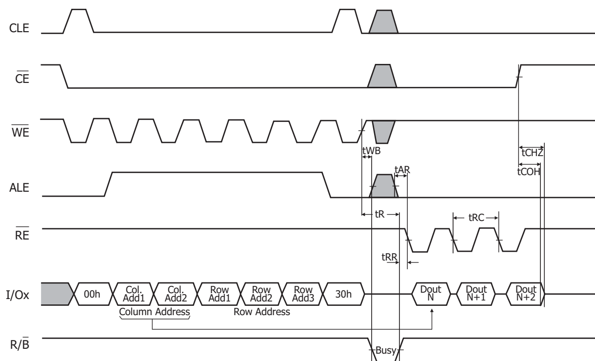
Figure 11: Read1 Operation intercepted by \overline{\text{CE}}
