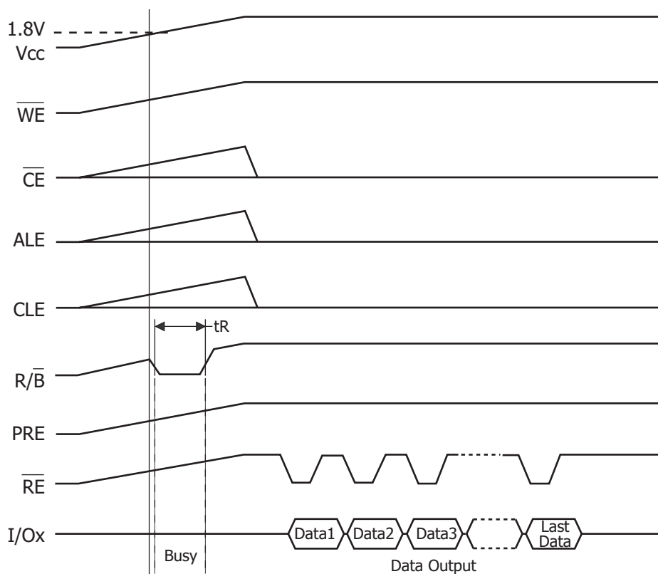
Figure 23: Automatic Read at Power On
