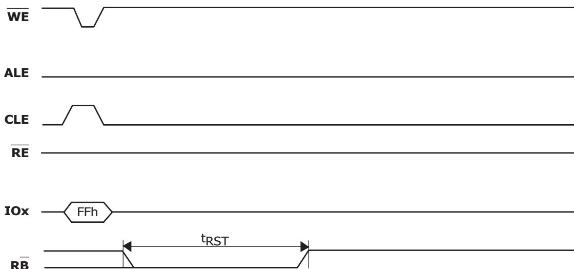
Figure 24: Reset Operation
