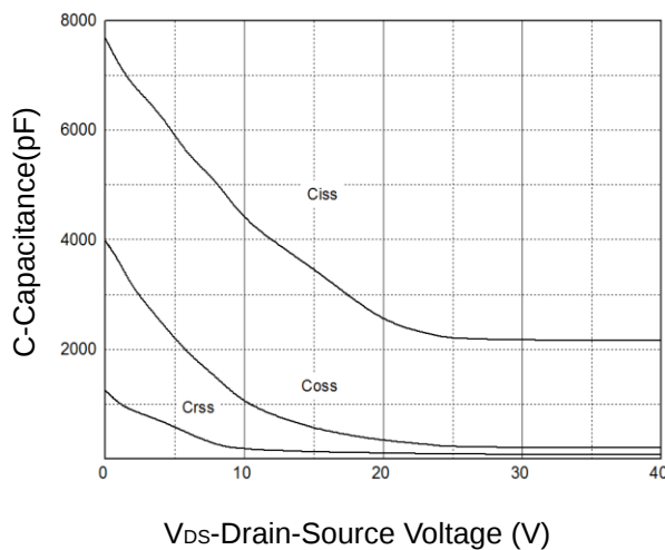
Figure 11: Capacitance Characteristics
