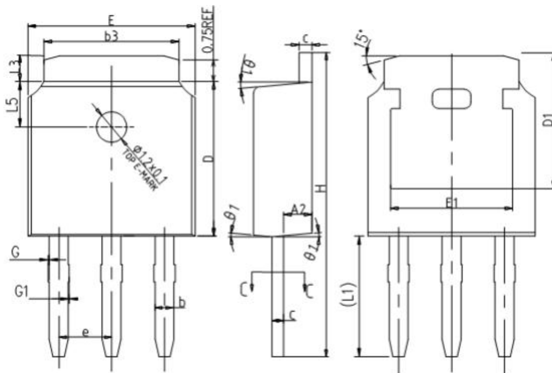
COMMON DIMENSIONS
