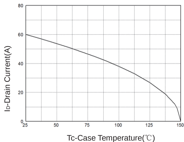
Figure 2: Drain Current
