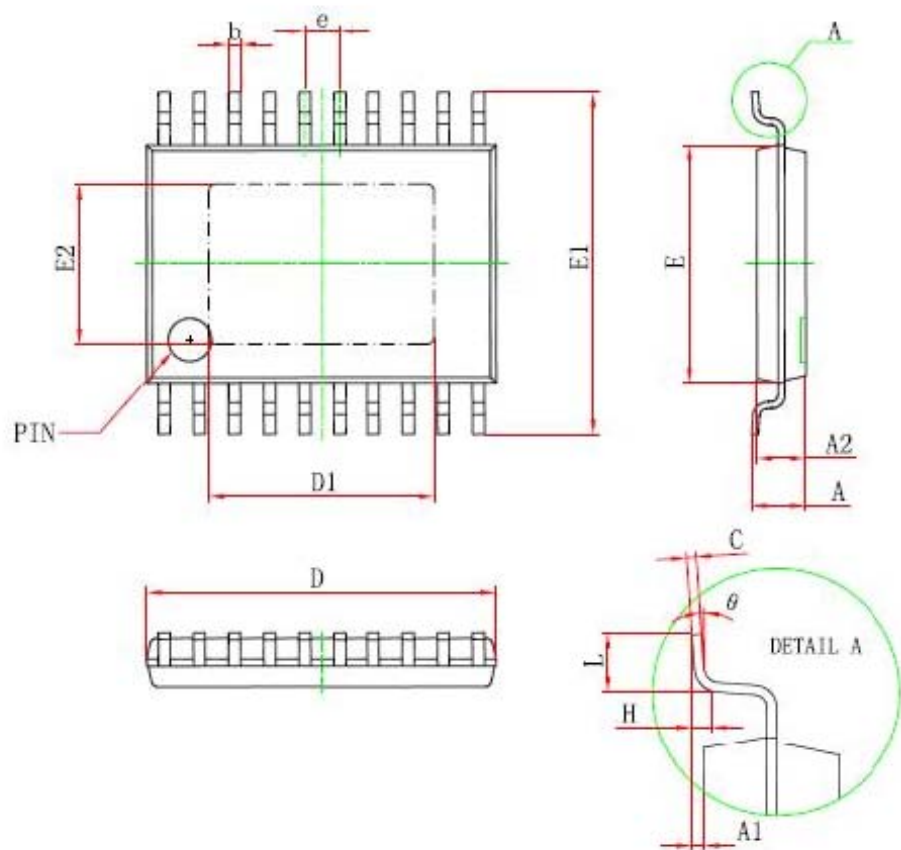
TSSOP20/PP PACKAGE OUTLINE DIMENSIONS
