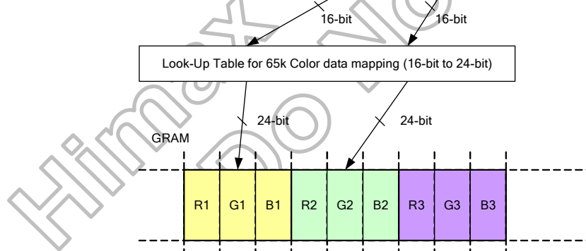
Figure 4.8: Write data for RGB 5-6-5 (65k colours) bit input in 18-bit parallel interface
