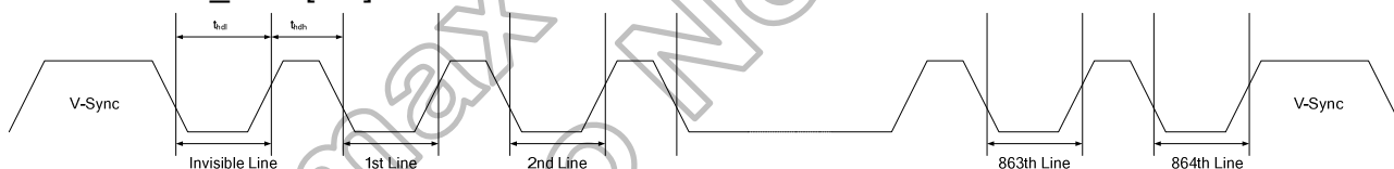
Figure 5.17: Tearing effect output line-mode 2
