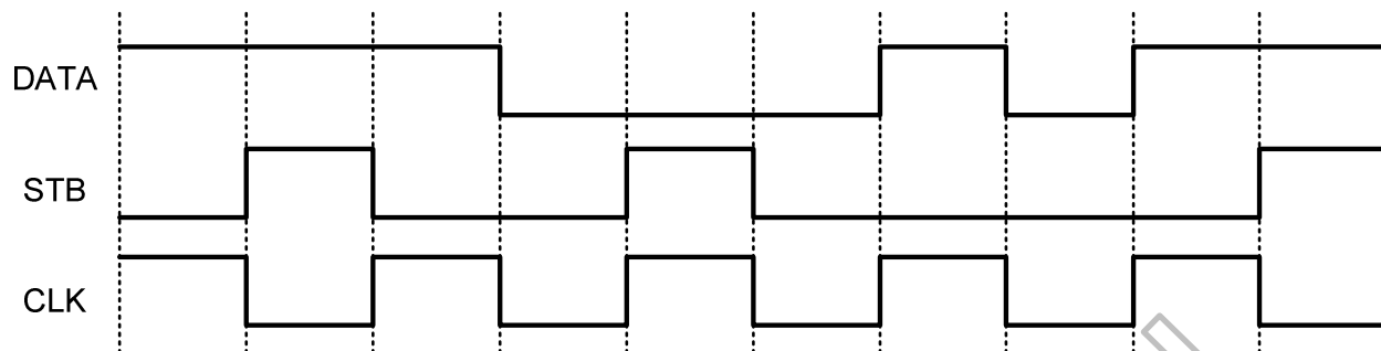
Figure 4.44: Data-STB encoding
