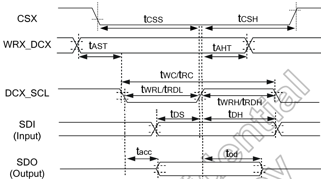
Figure 8.3: DBI Type C interface characteristics
