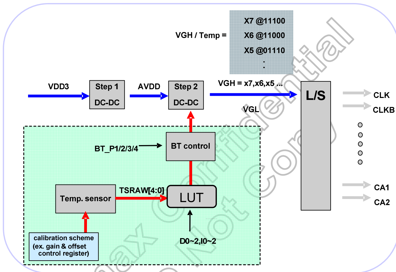
Figure 5.46: Temperature sensor
