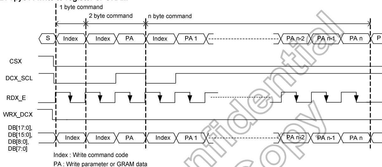
Figure 4.1: DBI-A system interface protocol, write to register or GRAM
