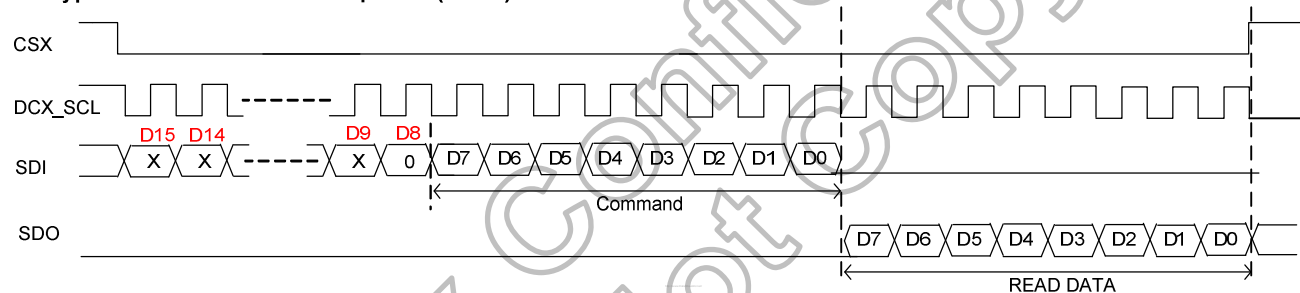
DBI Type-C Interface Protocol – Option 2 (3 wire)
