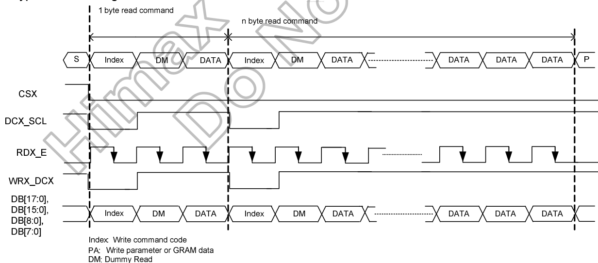
Figure 4.2: DBI-A system interface protocol, read from register or GRAM
