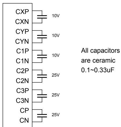
Figure 14. 1: Booster capacitors
