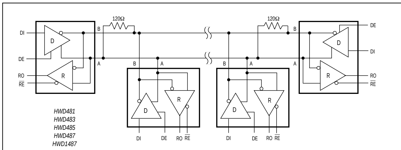
Figure 21. HWD481/HWD483/HWD485/HWD487/HWD1487 Typical Half-Duplex RS-485 Network
