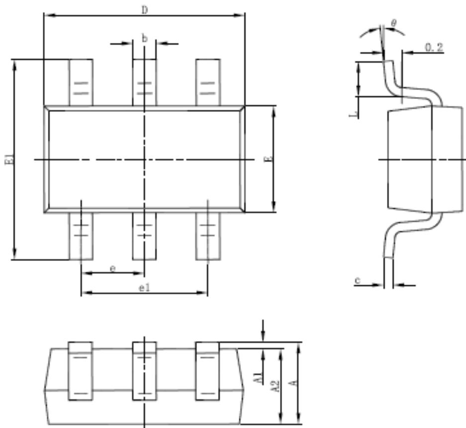
SOT-23-6L PACKAGE OUTLINE DIMENSIONS
