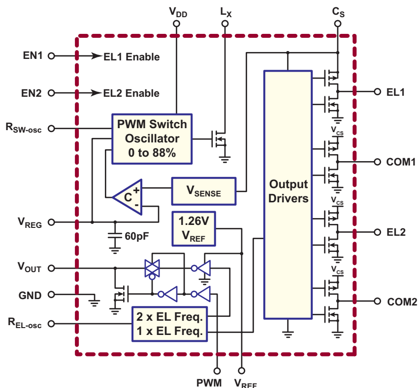
Figure 1: Block Diagram
