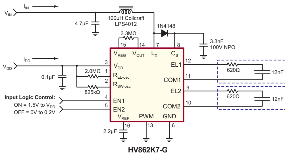
Figure 2: Test Circuit
