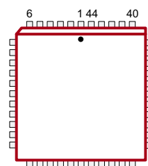
44-Lead PLCC
