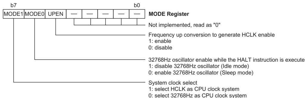
MODE Register
