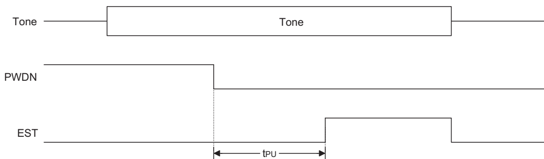
Power-up Timing
