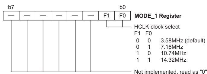
MODE_1 Register
