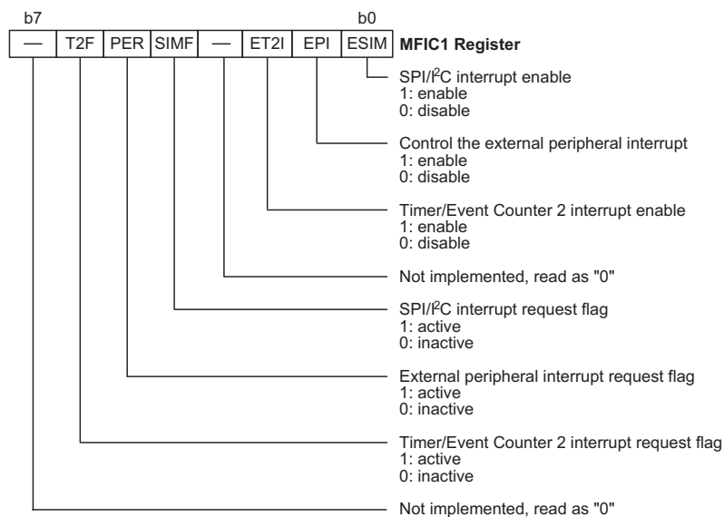
MFIC1 Register
