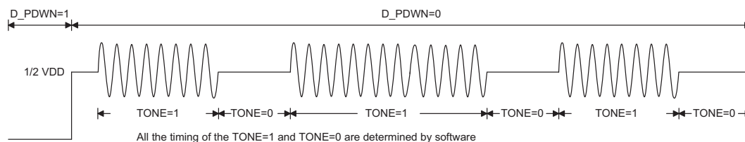
DTMF Output
