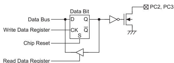
PC2, PC3 NMOS Output Port
