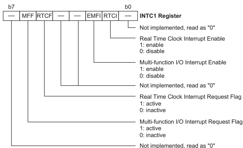
Interrupt Control 1 Register
