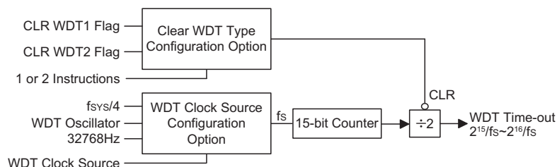
Watchdog Timer
