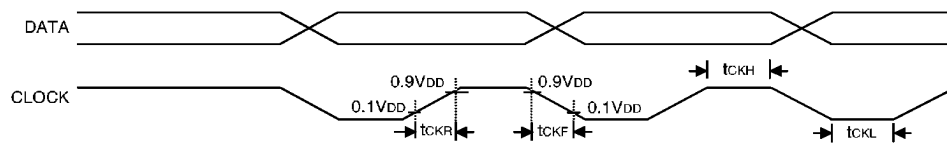
Figure 2. Programming timing
