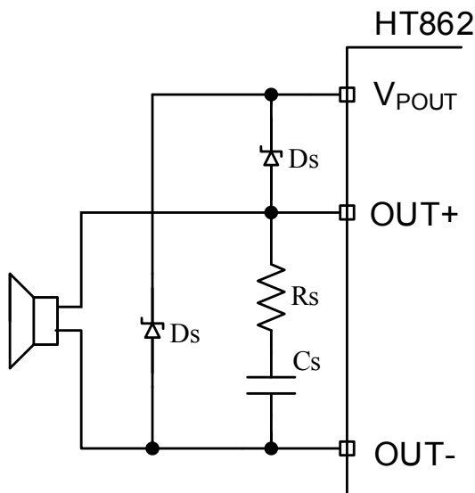
Fig. 11 Amplifier Output Configuration
