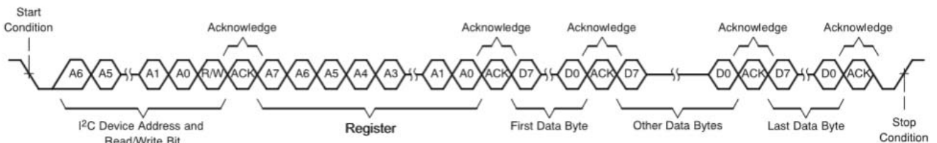
Fig. 14 Multiple-Byte Write Transfer
