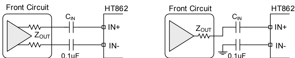
Fig. 10 (1) Differential Input;
