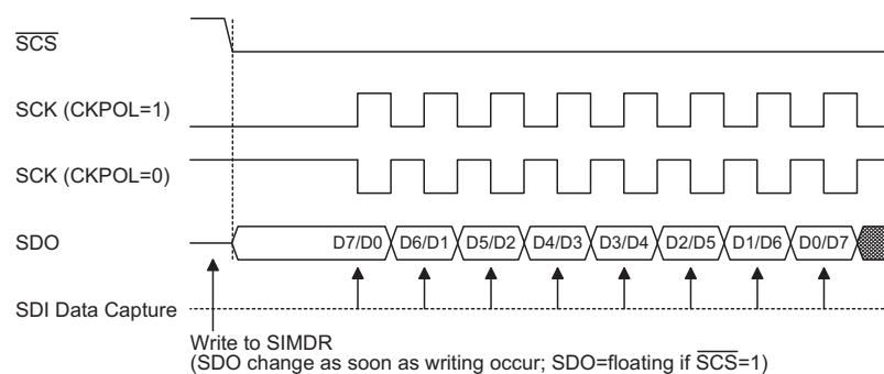
SPI Slave Mode Timing (CKEG=1)
