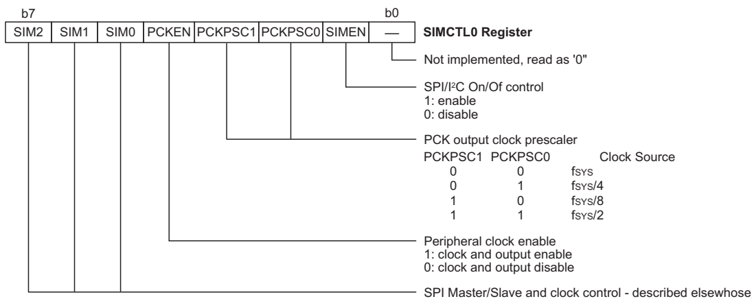
Peripheral Clock Output Control – SIMCTL0
