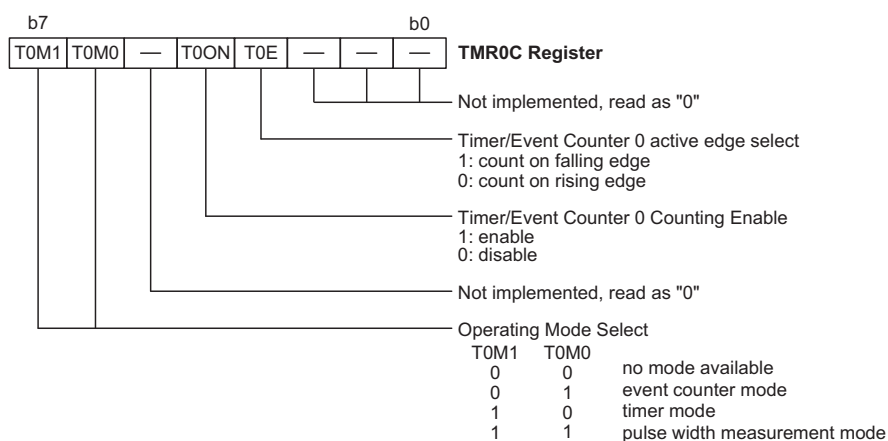
Timer/Event Counter 0 Control Register
