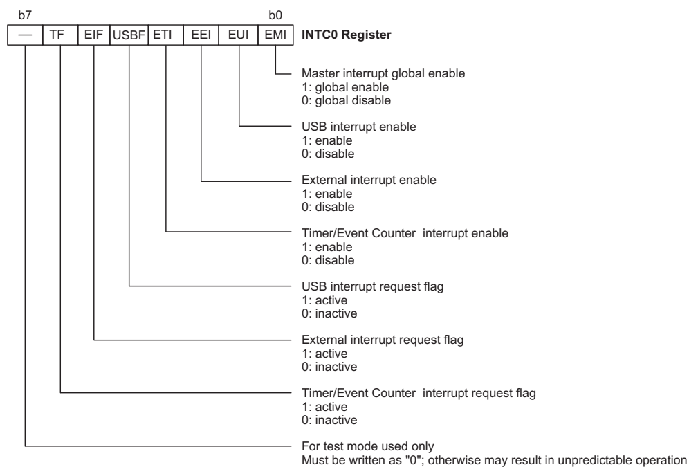
INTC0 Register
