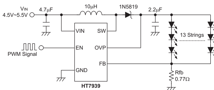
Figure 14. Application Circuit for Dimming Control Using a PWM Logic Signal
