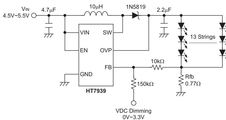
Figure 15. Application Circuit for Dimming Control Using a DC Voltage
