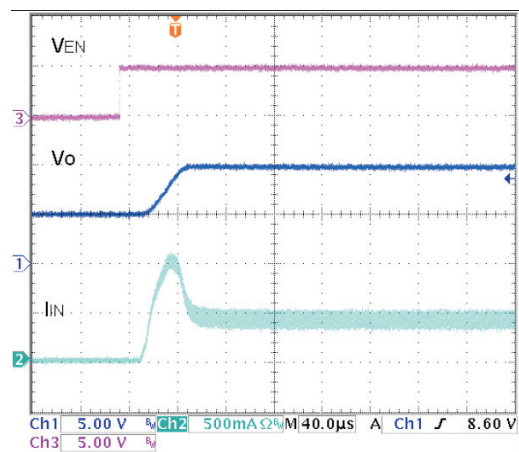
Fig.9 Start-up Waveform
