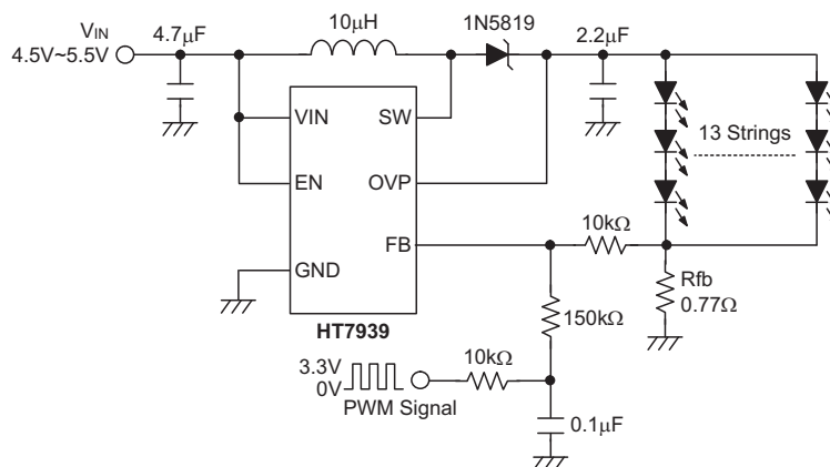
Figure 16. Application Circuit for Dimming Control Using a Filtered PWM Signal
