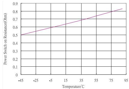
Fig.7 RDS(ON) VS Temperature
