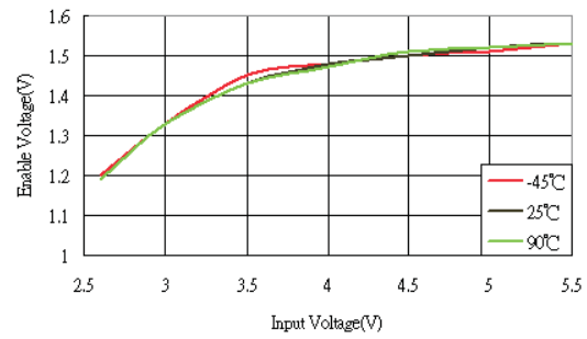
Fig.5 Enable Voltage VS Input Voltage
