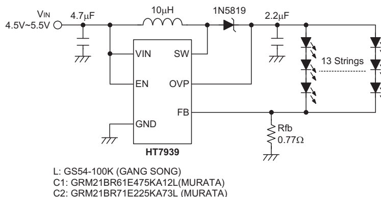
Figure 13. Application Circuits for Driving 39 WLEDs
