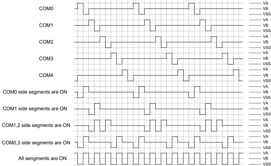
LCD Driver Output – Type A, 1/5 Duty, 1/2 Bias
