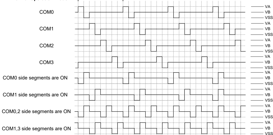
LCD Driver Output – Type A, 1/4 Duty, 1/2 Bias
