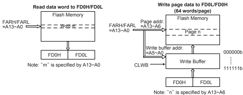
Flash Memory IAP Read/Write Structure – HT66FB572
